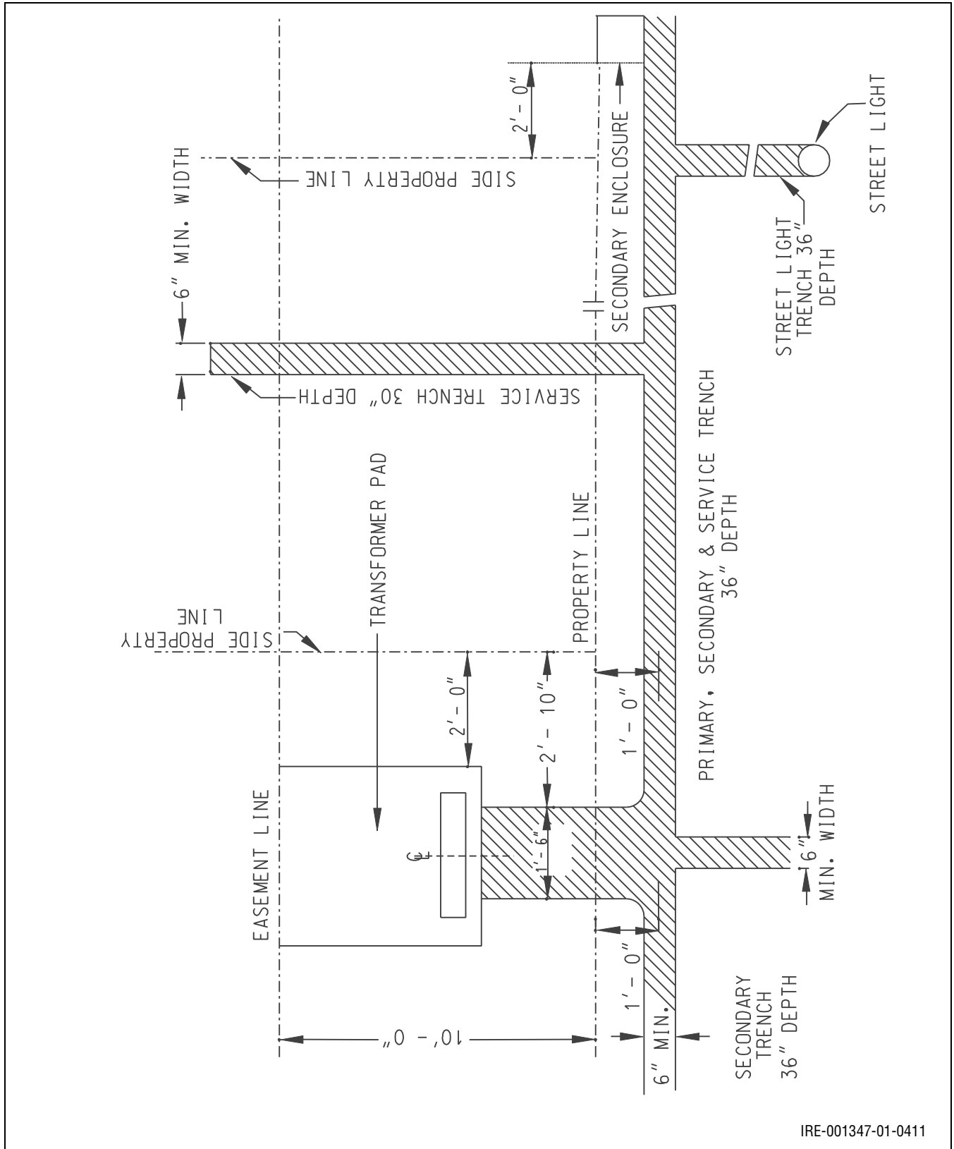
Figure 10.37: Single-Phase Padmounted Transformer Pads
