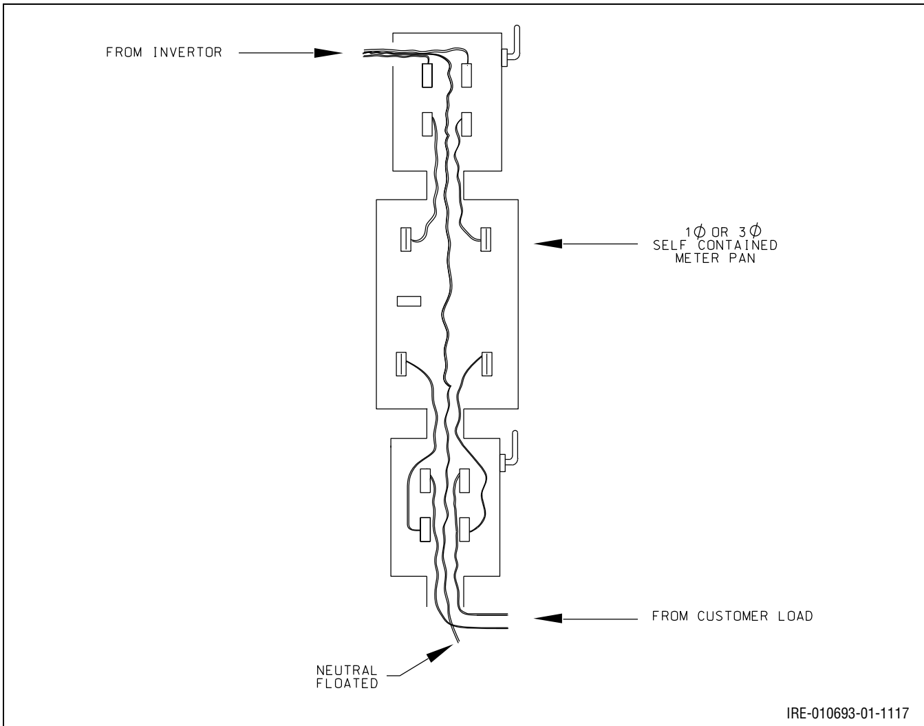
Figure 9.2: Self-Contained Residential Solar Loan Wiring Configuration
