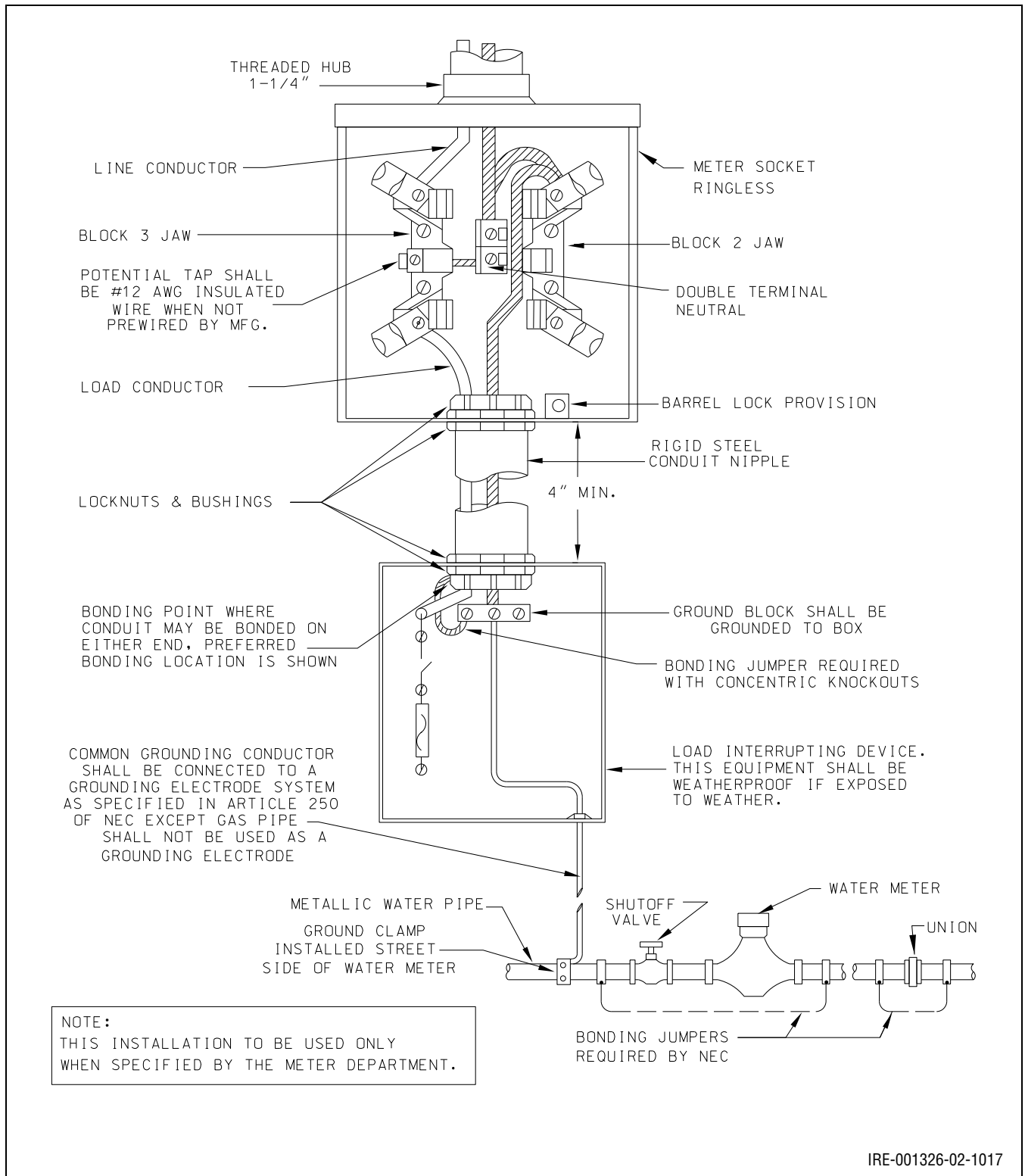
Figure 10.15: Single-Phase, Two-Wire 120 V for Two-Wire Socket Meter
