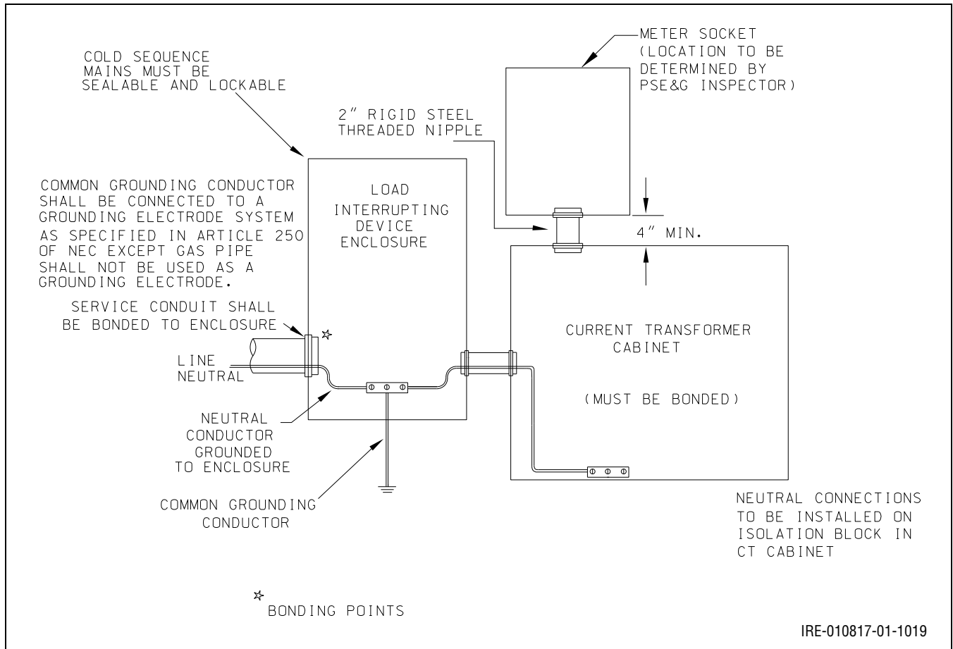
Figure 10.25: Grounding and Bonding CT Enclosure – Cold Sequence Bar Type CT
