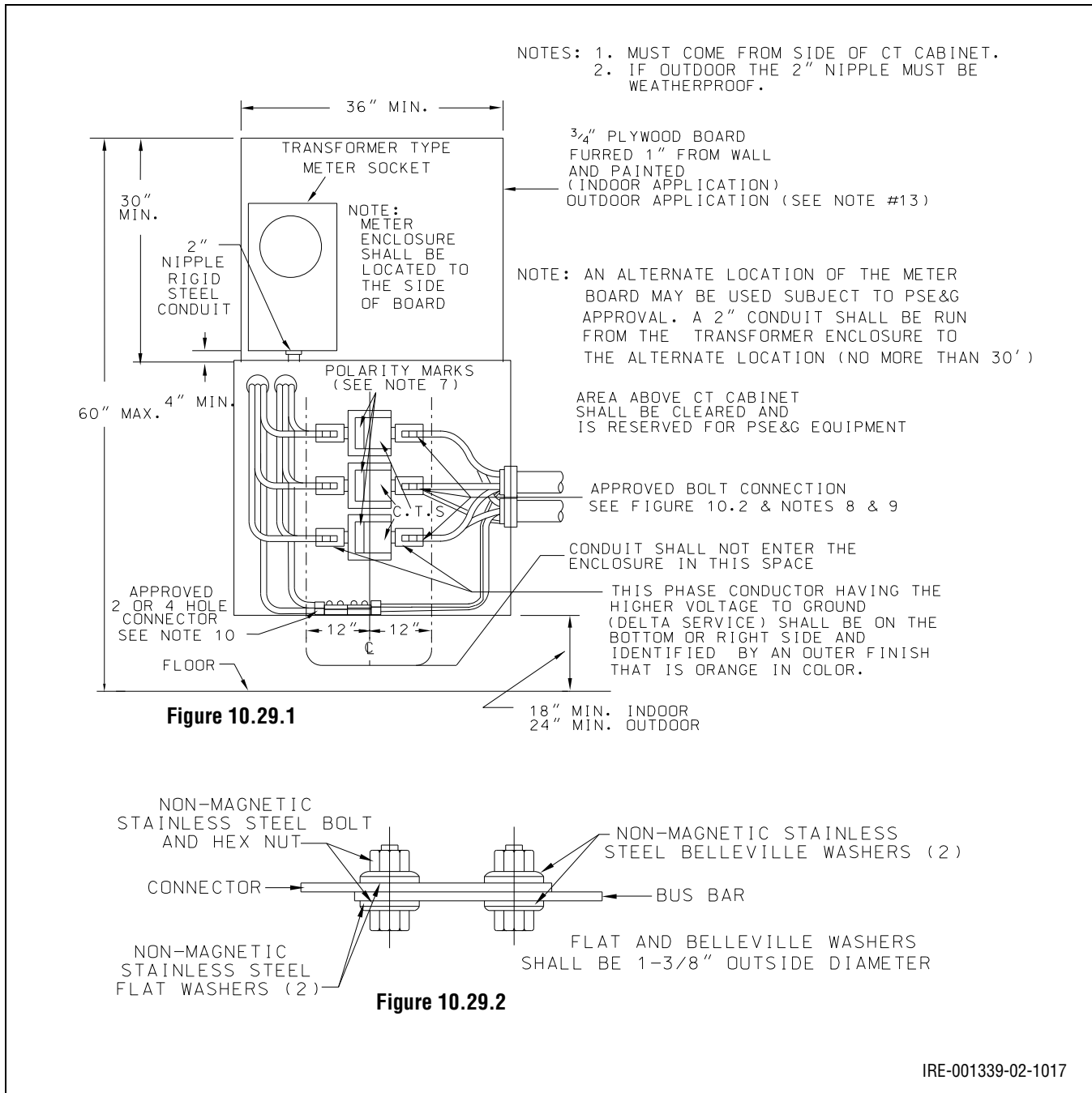
Figure 10.29: Maximum Capacity Parallel 500 kcmil Conductors – Three-Phase Four- Wire Service
