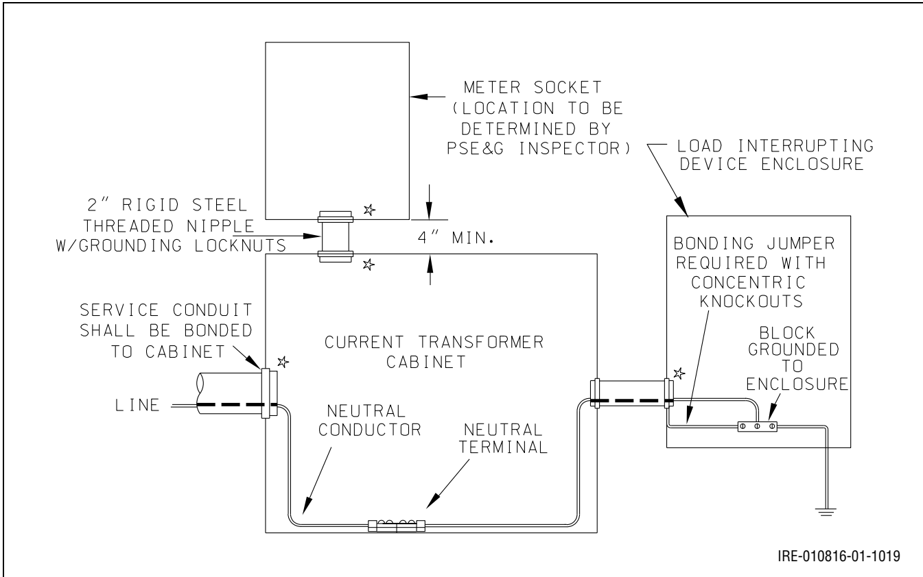
Figure 10.24: Grounding and Bonding CT Enclosure – Hot Sequence, Bar Type CT
