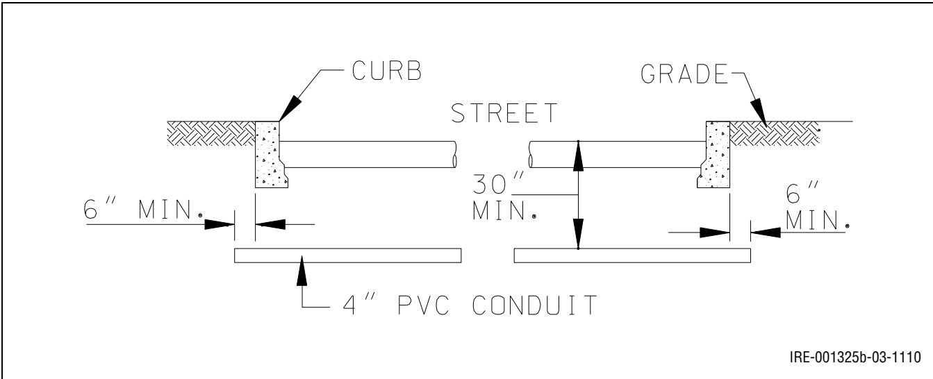
Figure 10.14: Standard Trenches
