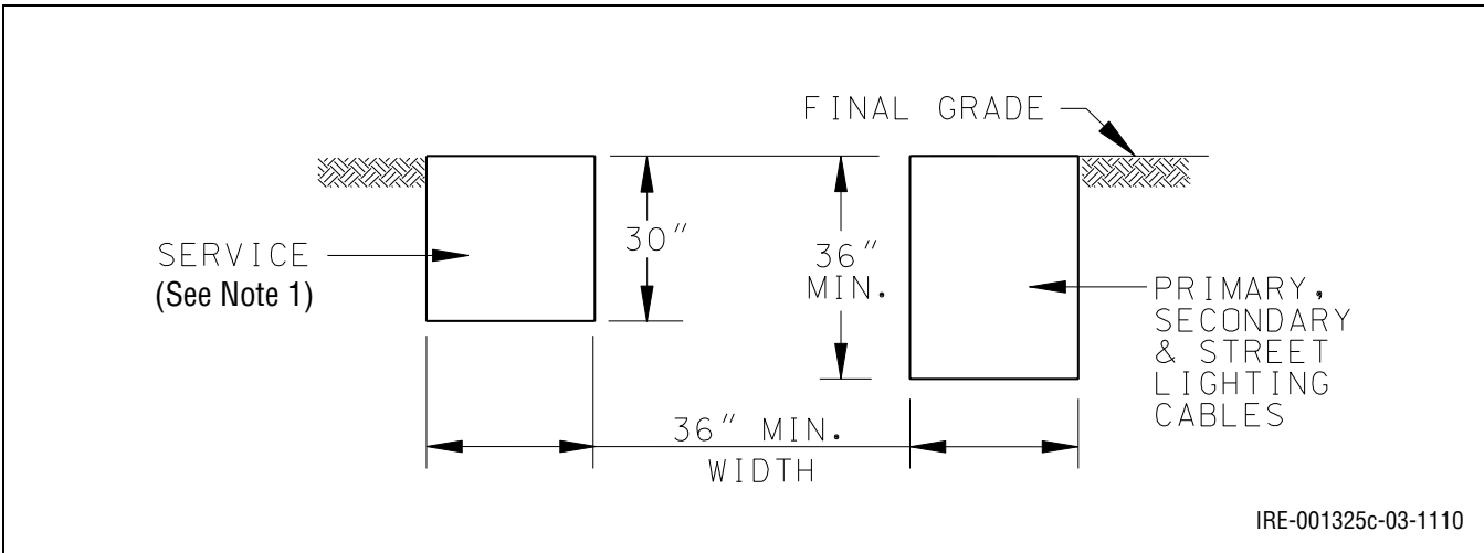
Figure 10.14: Standard Trenches
