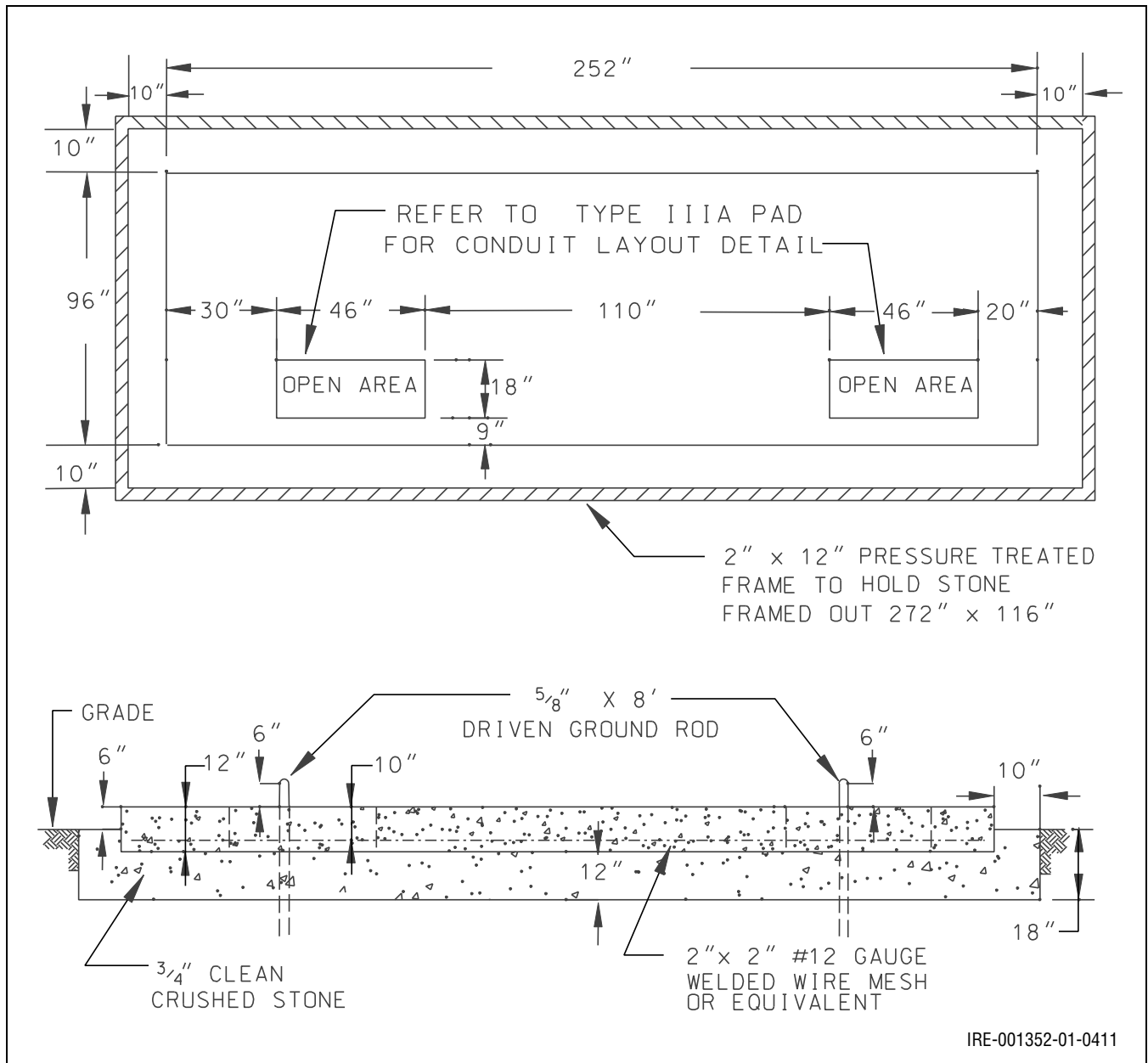
Figure 10.42: Three-Phase Padmounted Transformer – Type V-A (Concrete)
