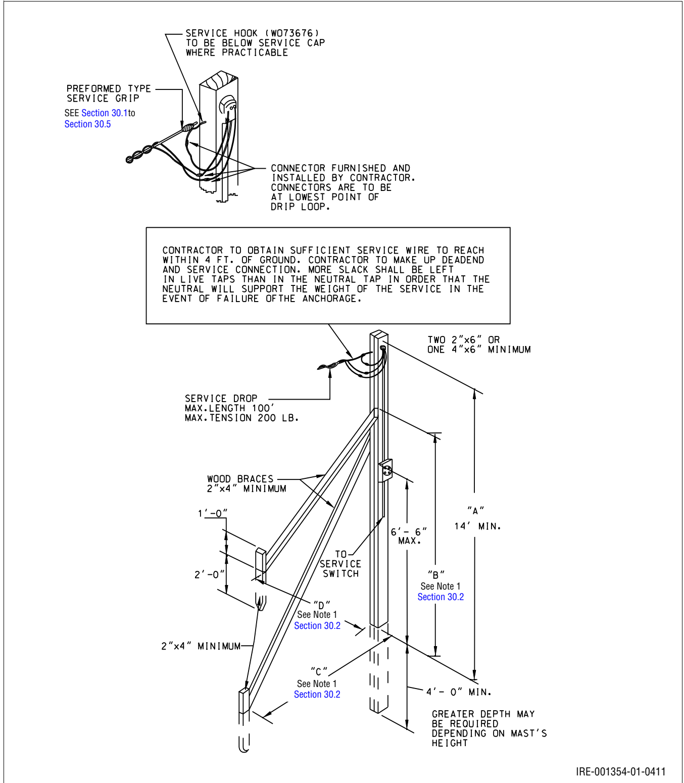
Figure 10.47: Minimum Requirements for a Temporary Service Mast
