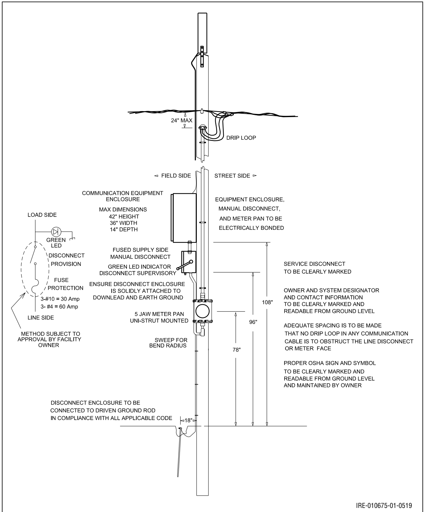
Figure 10.53: Metered Installation for third Party Equipment on Secondary Distribution Pole
