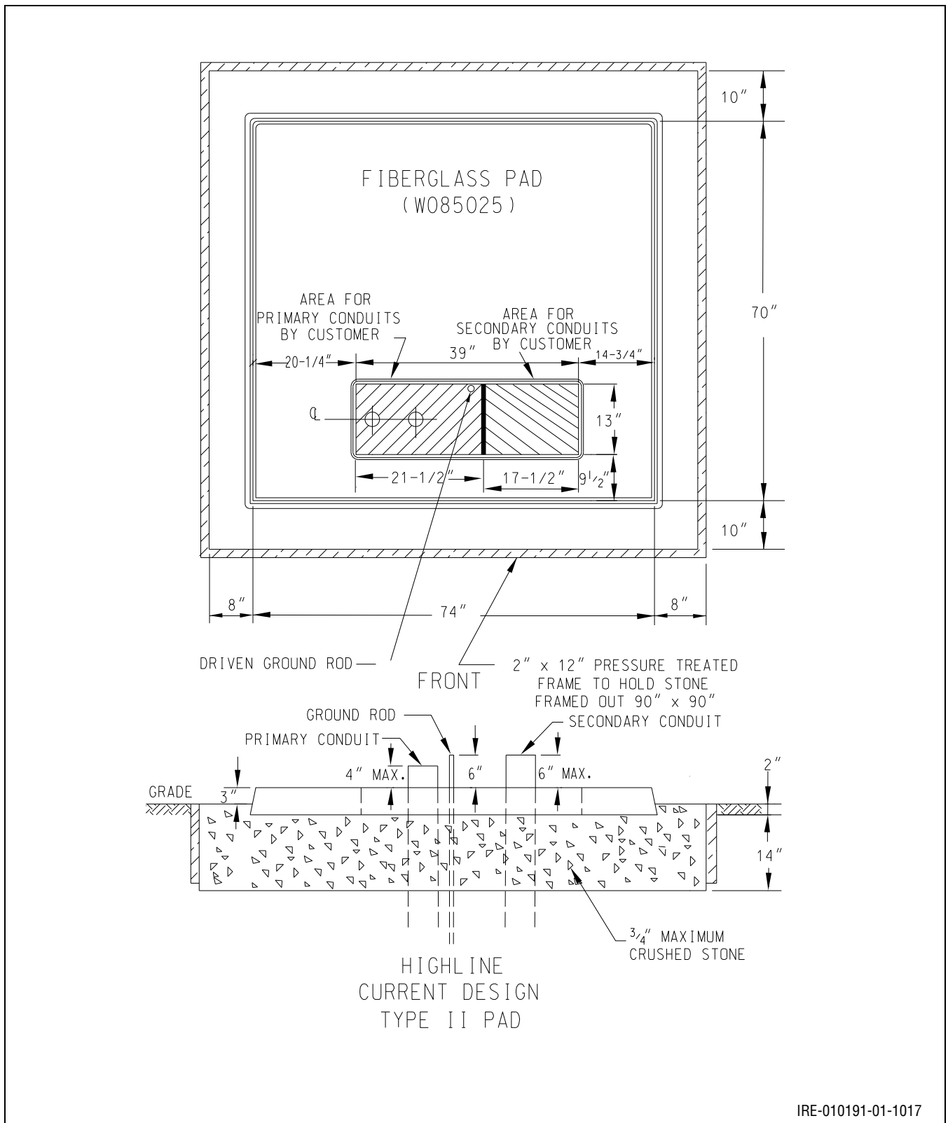
Figure 10.39: Fiberglass Pad Three-Phase Padmounted Transformers (300 kVA and below) – Type II (Highline Current Design Type II Pad)
