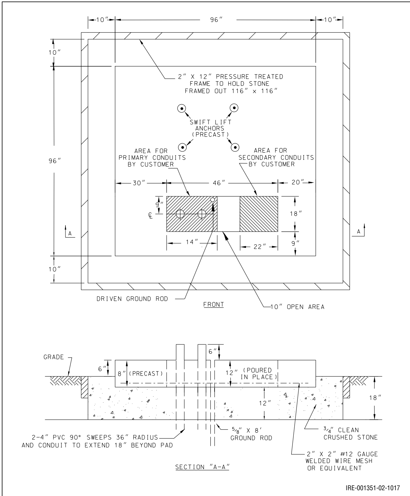
Figure 10.41: Three-Phase Padmounted Transformer – Type III-A (Concrete)
