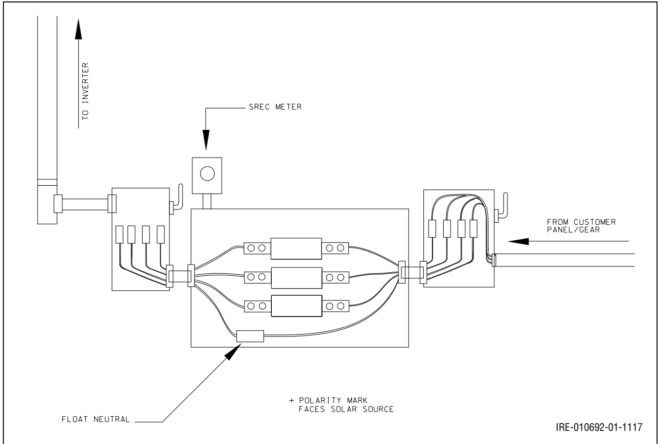
Figure 9.1: Current Transformer Rated Solar Loan Configuration
