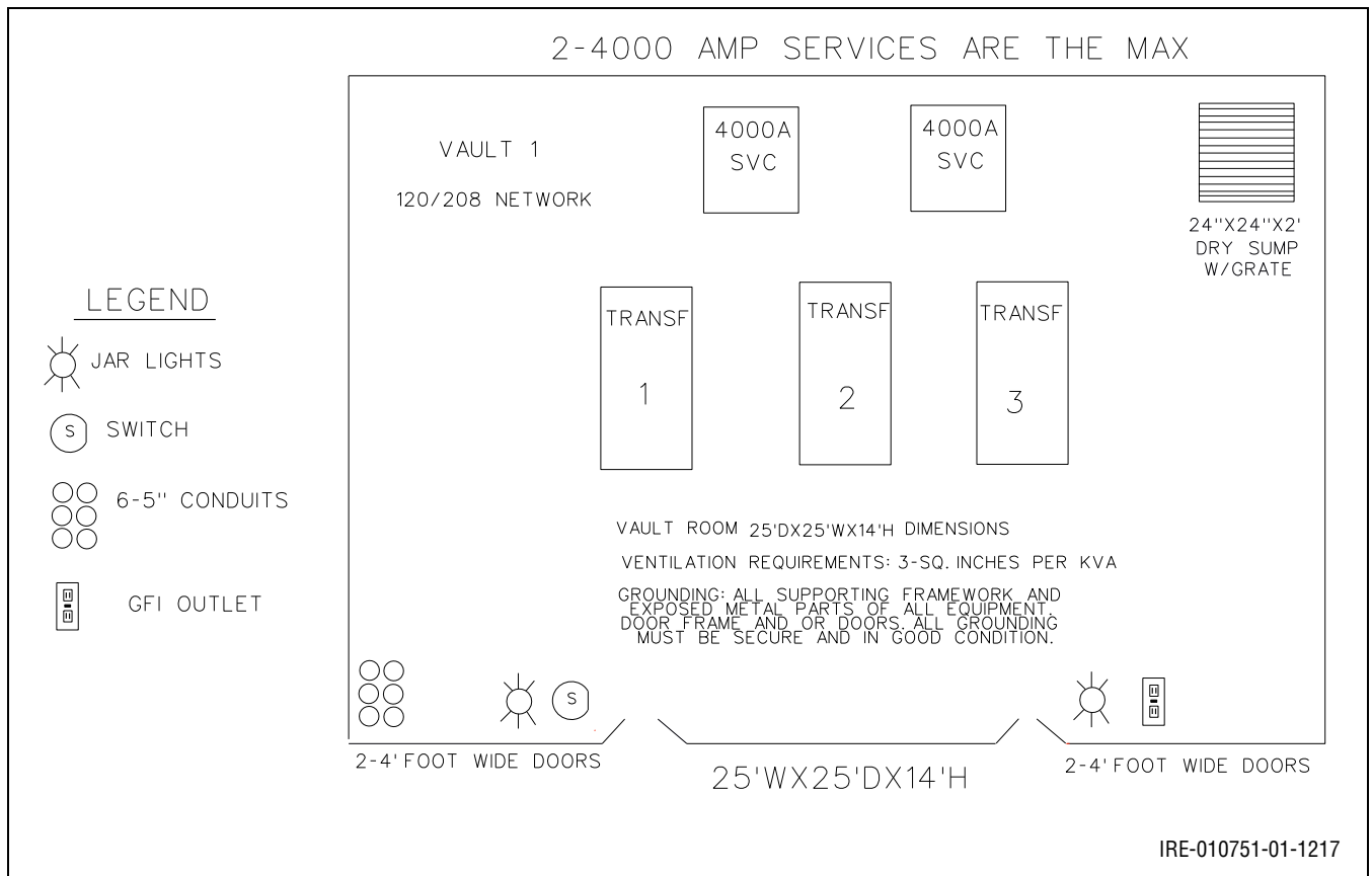
Figure 10.45: Network Vault Specifications – 120-208 V
