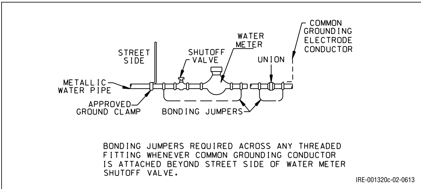
Figure 10.5: Grounding to Water System
