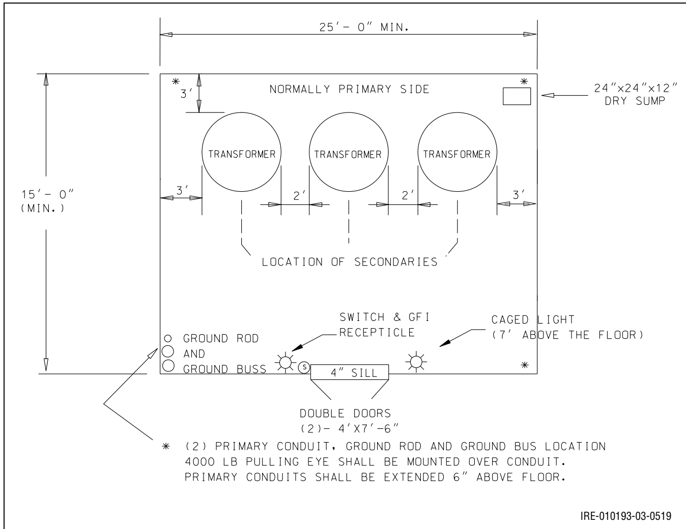
Figure 10.43: Transformer Vault Minimum Construction Dimensions Single – Up to Three 500 kVA Transformers
