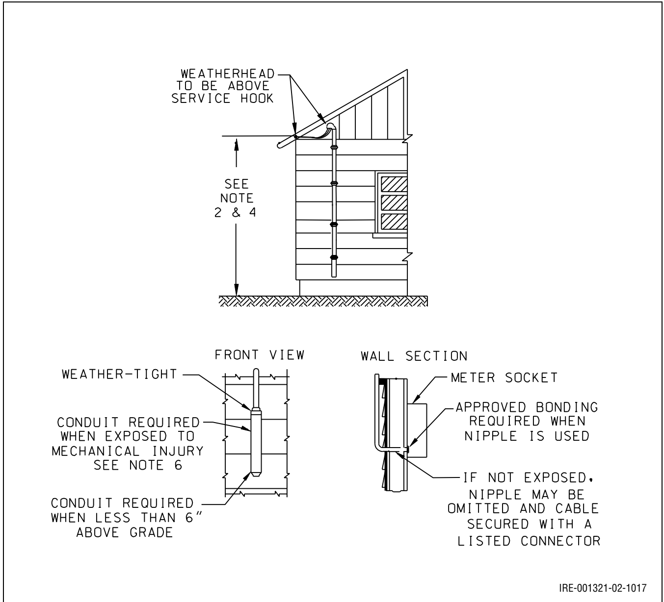
Figure 10.7: Non-Standard Installation – Special Approval Required – First Floor Installation
