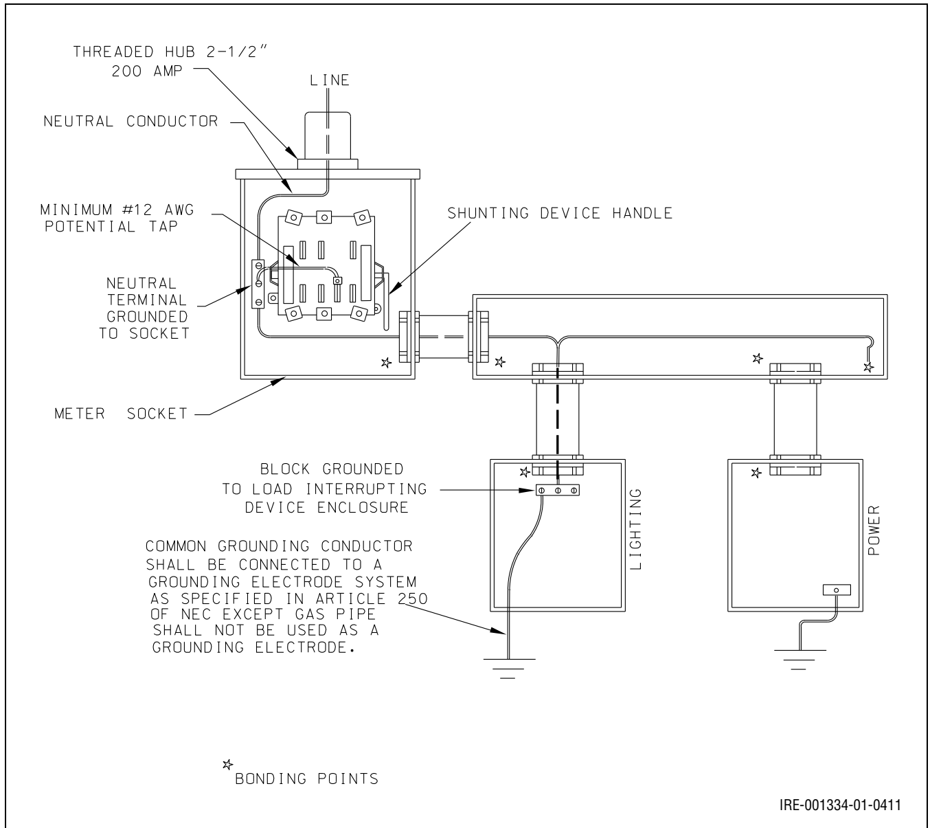
Figure 10.23: Combination Power and Light (4 W Delta Service)
