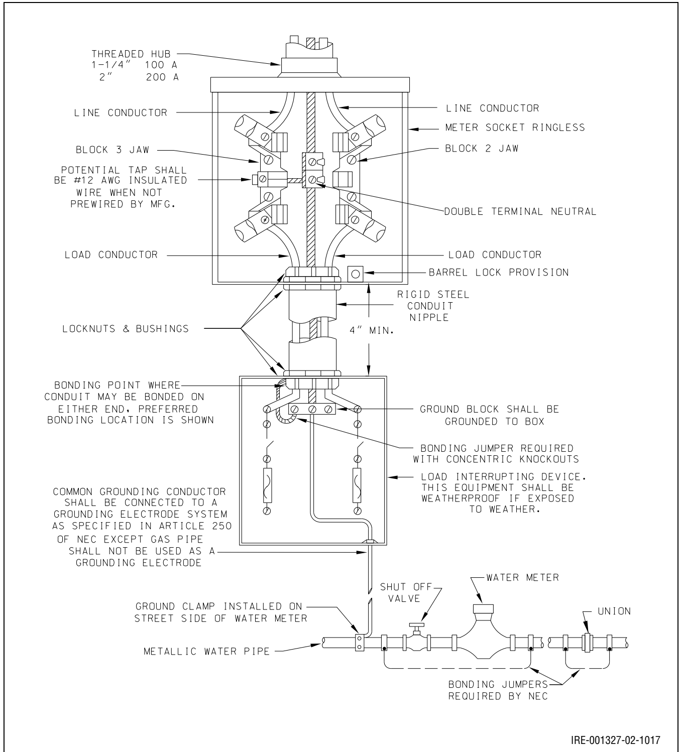
Figure 10.16: Single-Phase, Three-Wire, 120/208 or 120/240 V Three-Wire Socket Meter
