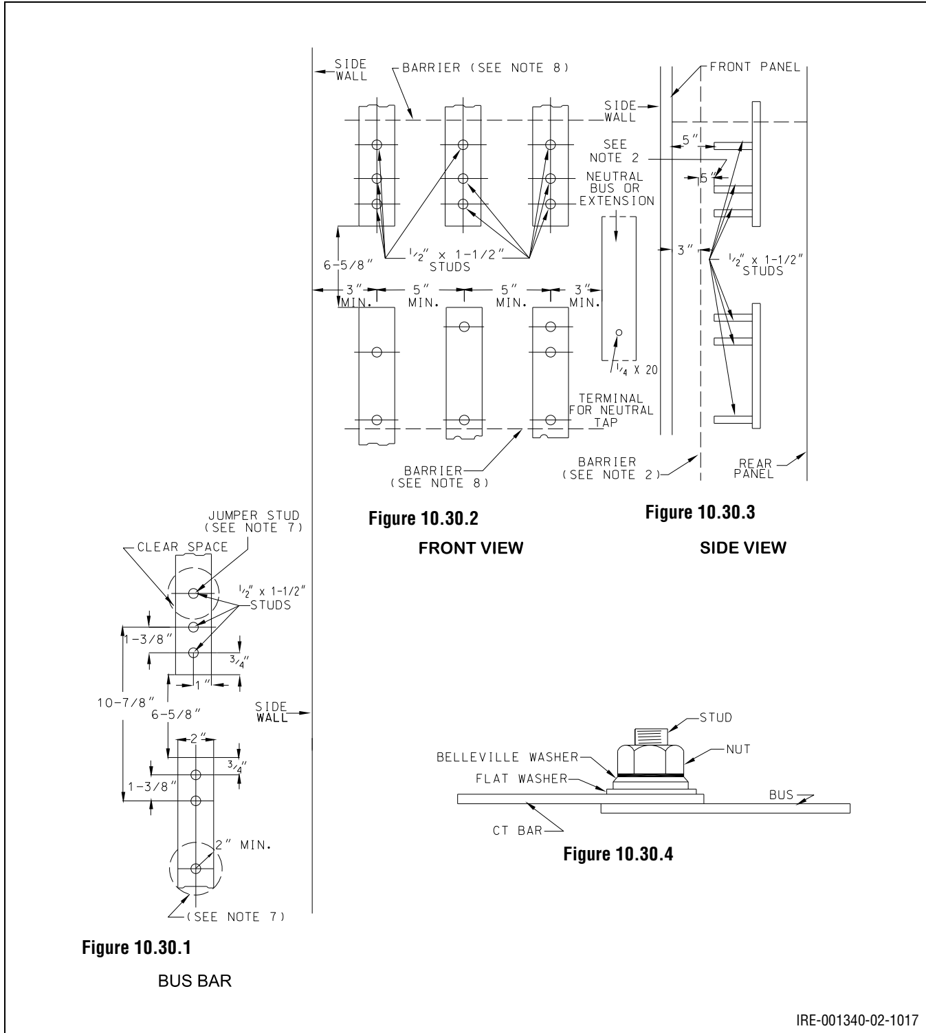
Figure 10.30: Minimum Clearances and Bus Arrangement for Bar Type Current Transformers 200 to 800 A Secondary
