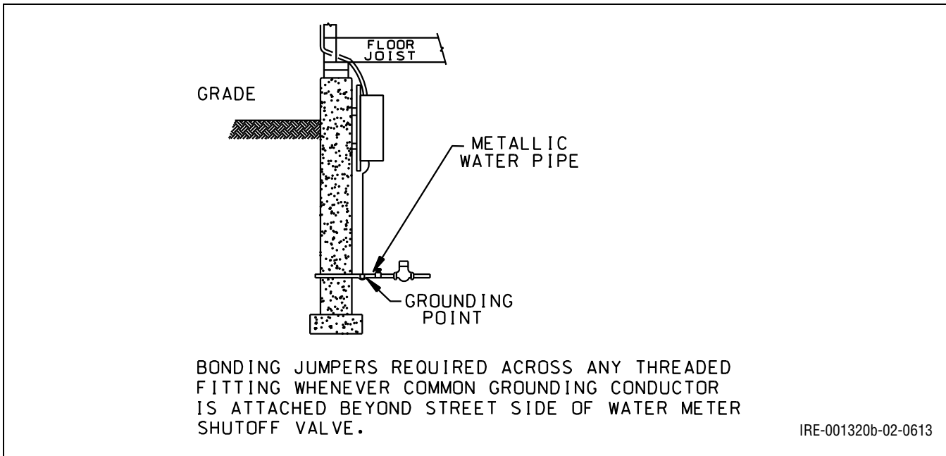
Figure 10.5: Grounding to Water System
