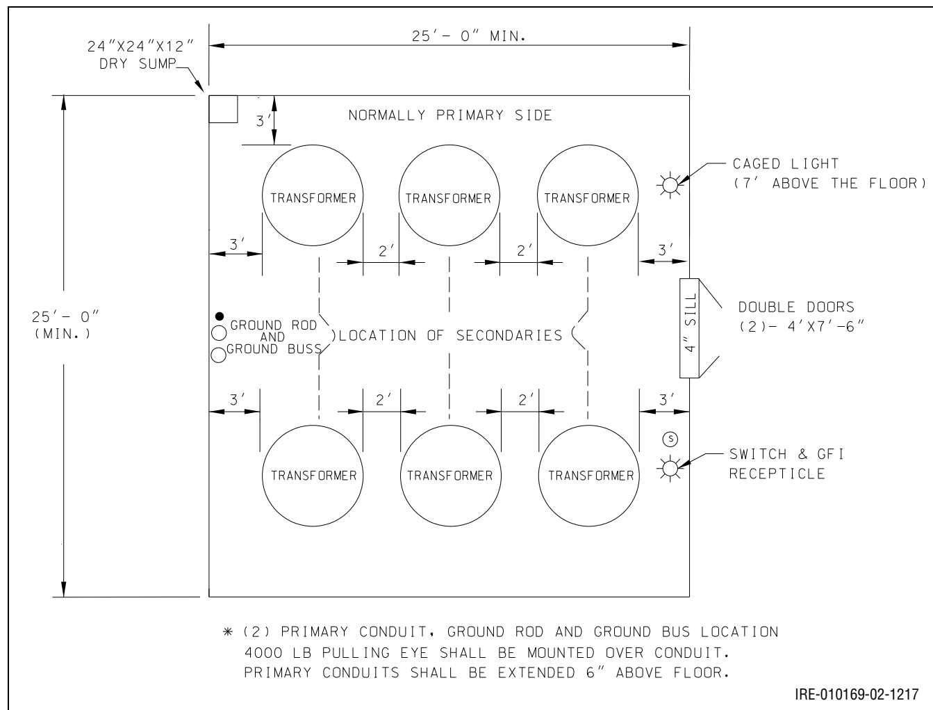
Figure 10.44: Transformer Vault Minimum Construction Dimensions Single – Up to Three 500 kVA Transformers Double – Up to Six 500 kVA Transformers
