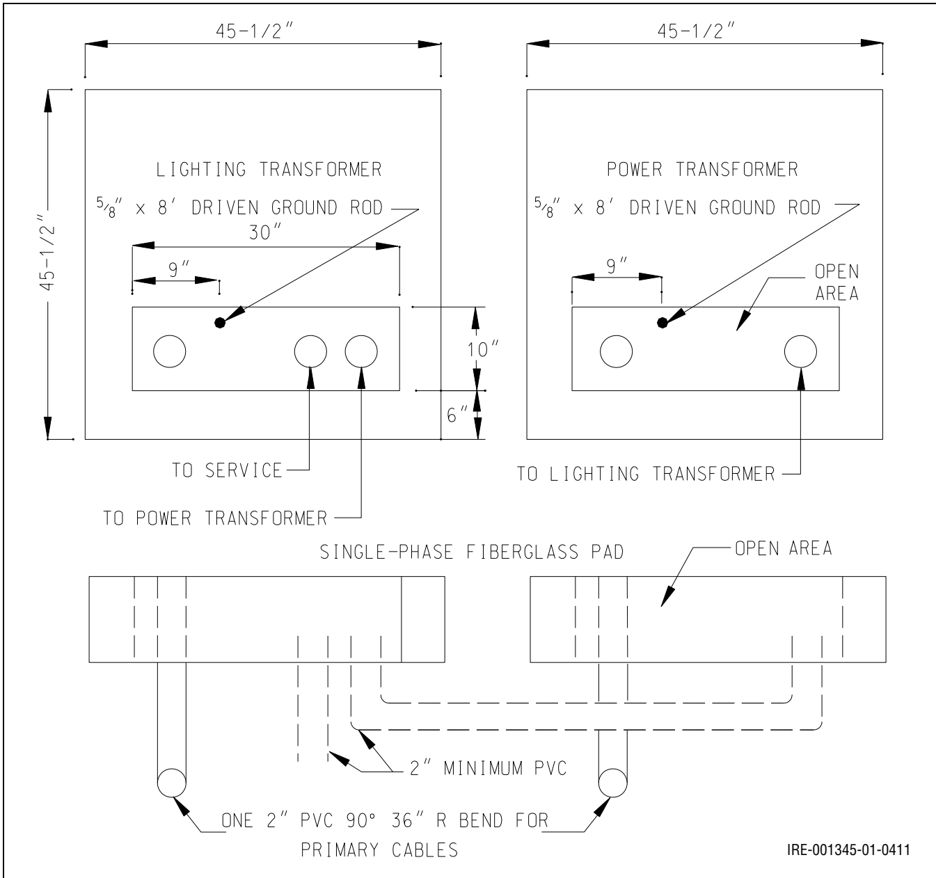
Figure 10.35: Secondary Conduit Connections for Single-Phase Open Delta Transformer
