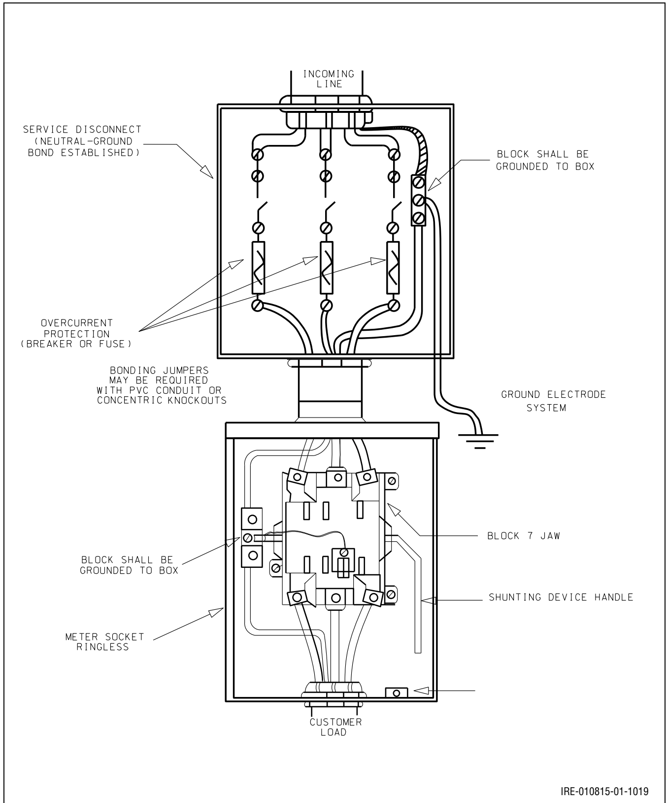
Figure 10.19: Three-Phase Four-Wire Services, Voltages Greater than 250 V (Cold Sequence)
