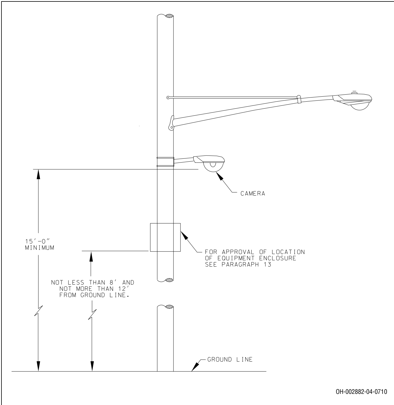
Figure 6.1: Closed Circuit Camera Attachments to Street Light Poles (Wood)
