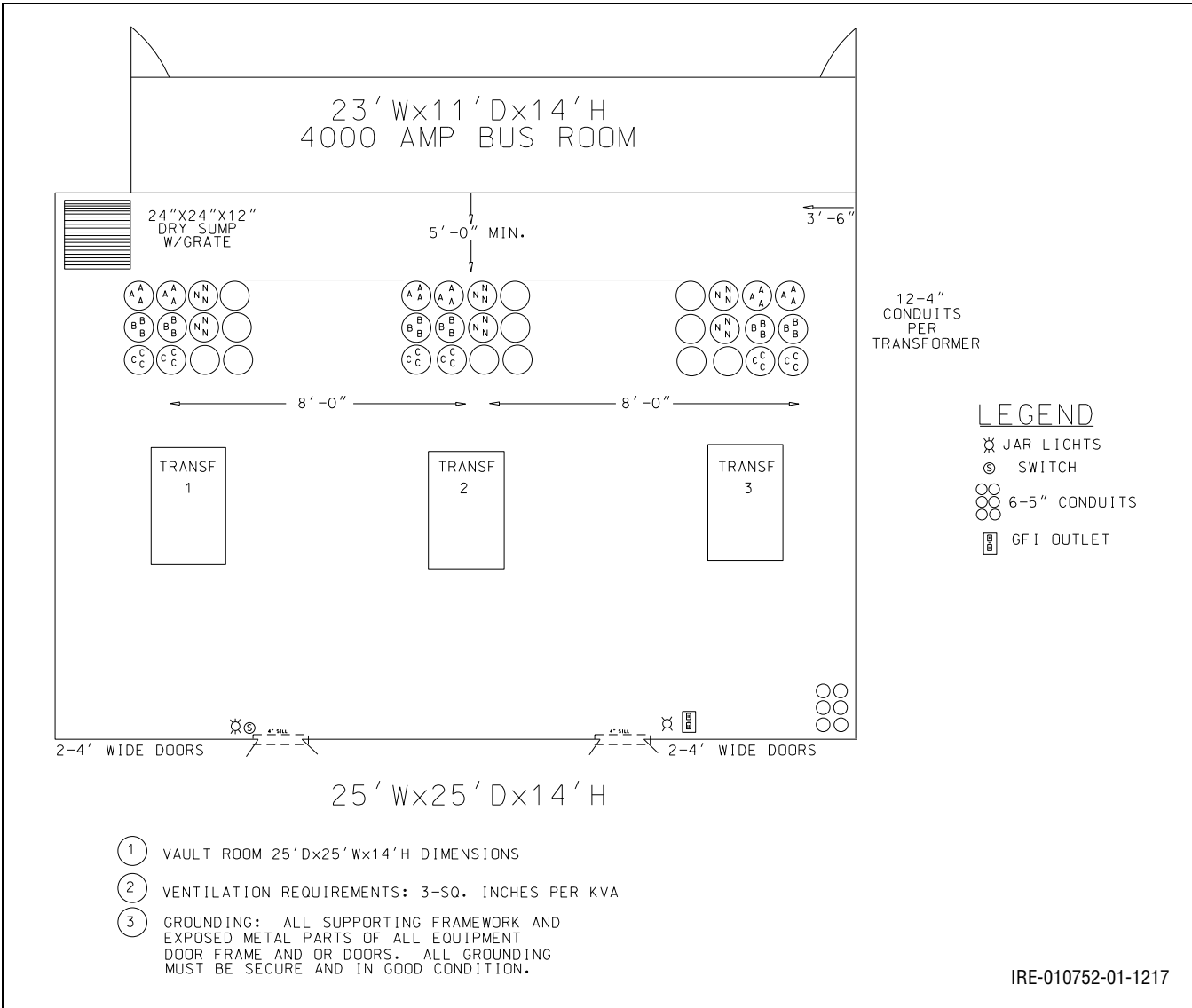
Figure 10.46: Network Vault Specifications – 277-480 V
