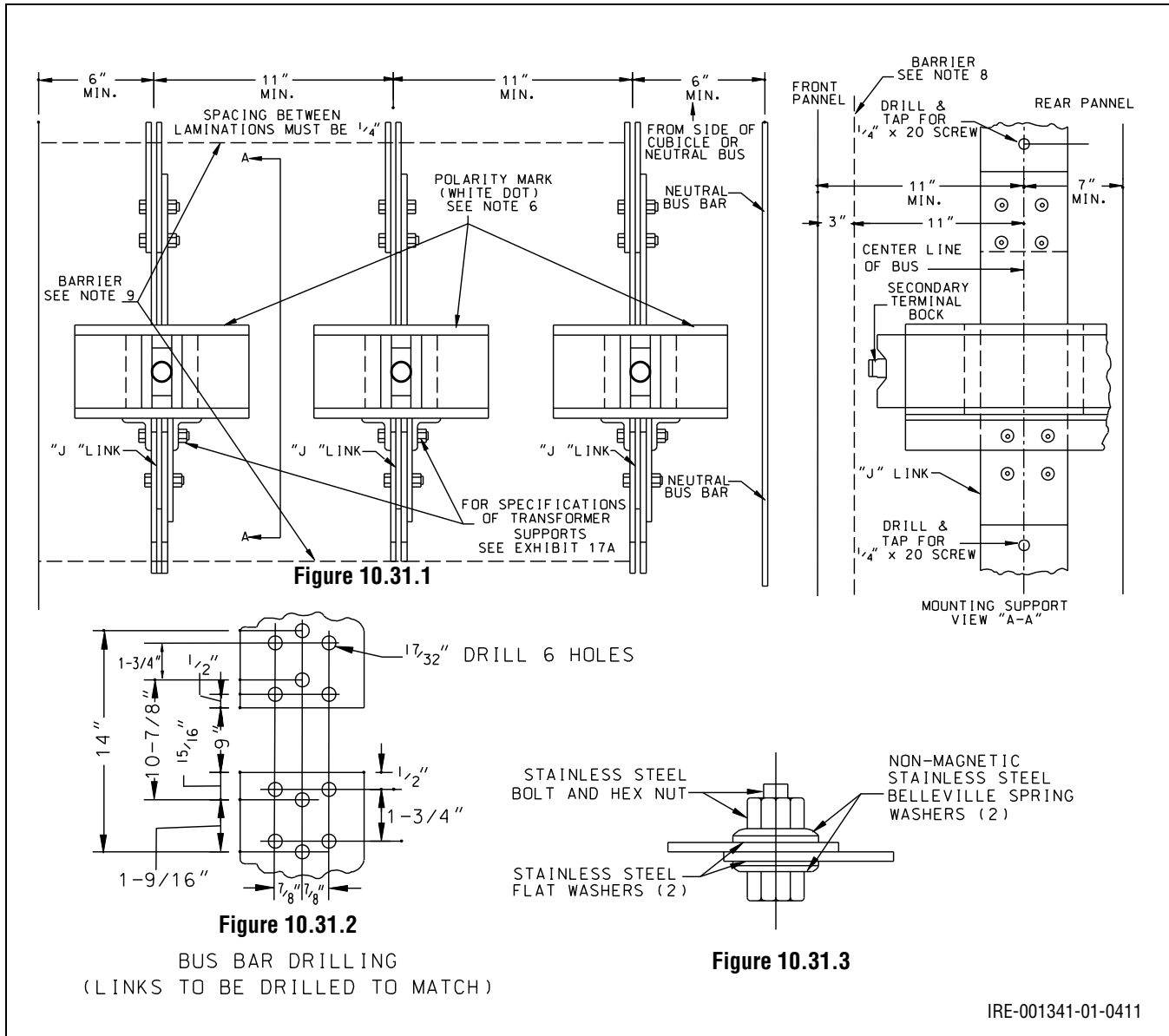
Figure 10.31: Mounting Dimensions for Current Transformers in Cubicle – Window Type >801 A to 4000 A Secondary
