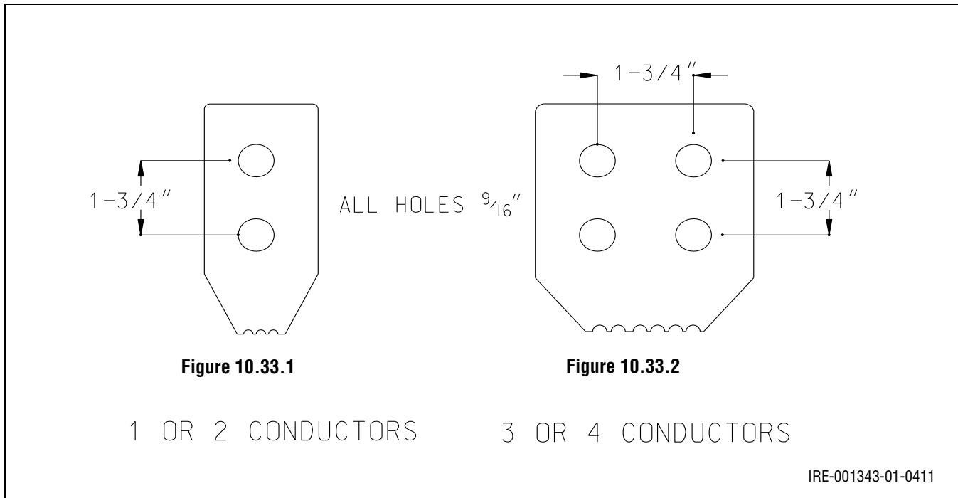
Figure 10.33: Secondary Connections to Terminals of PSE&G Equipment
