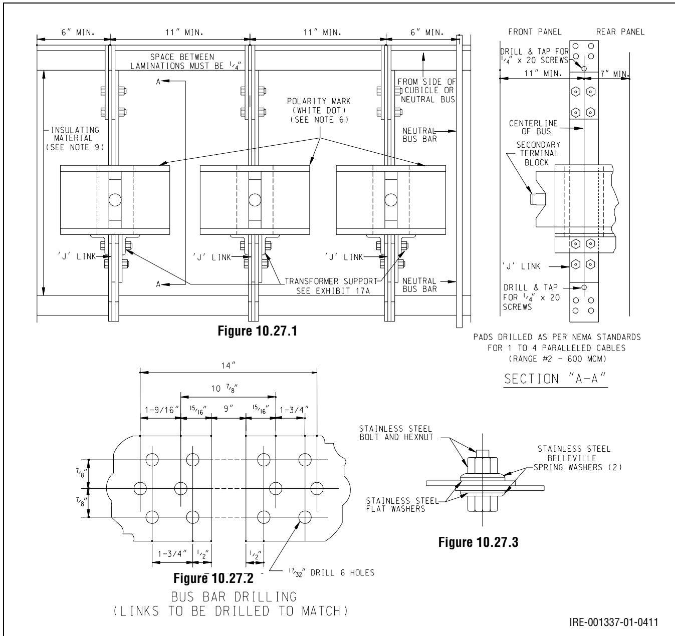
Figure 10.27: Window Type >801 A Secondary
