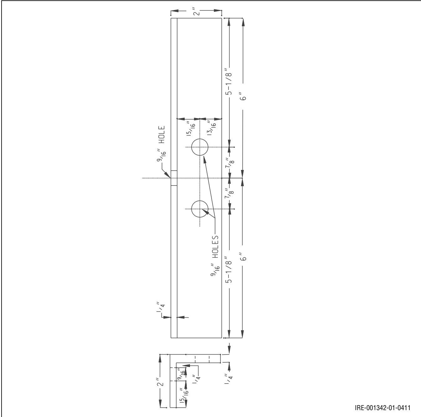
Figure 10.32: Current Transformer Mounting Bracket Specifications and Dimensions
