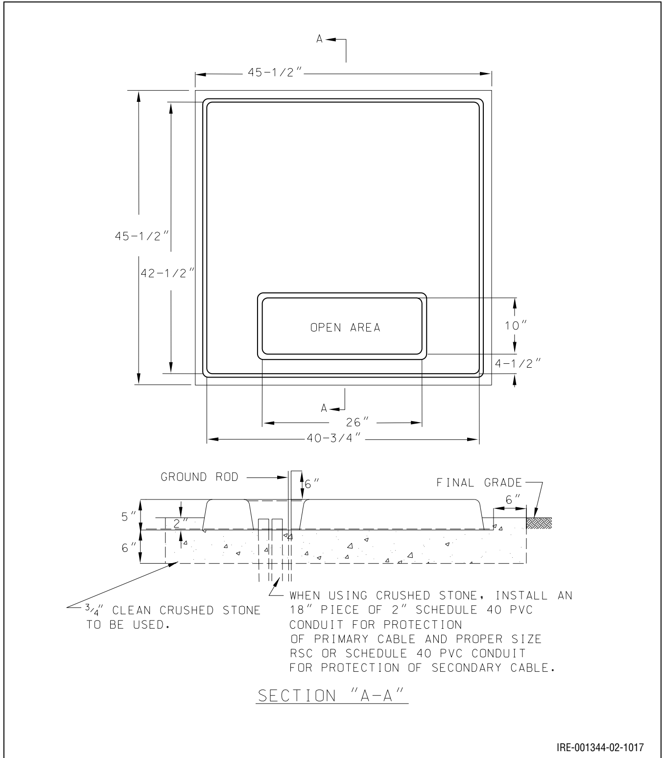
Figure 10.34: Fiberglass Pad – Present Design Single-Phase
