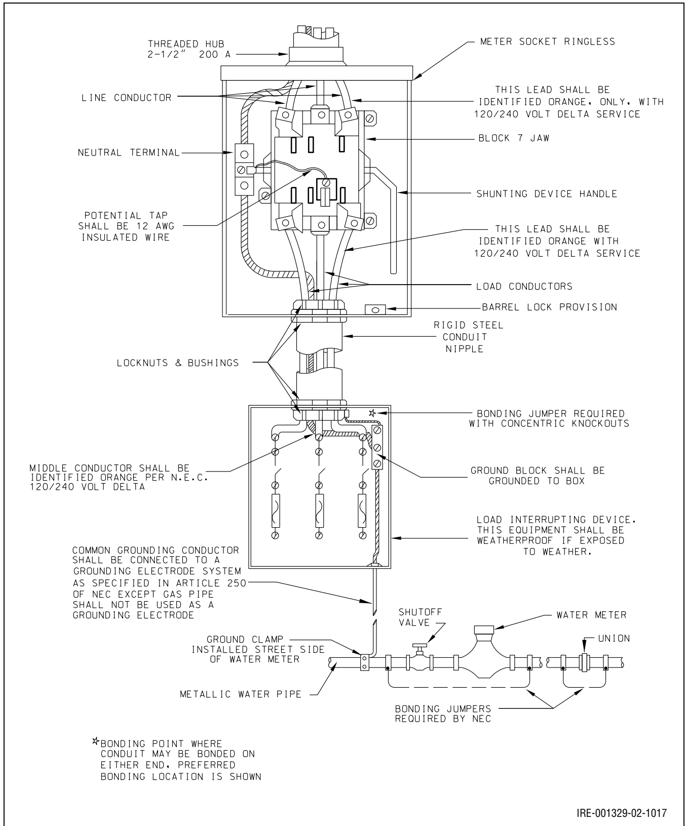
Figure 10.18: Three-Phase, Four-Wire Services – Voltage Less than 250 V
