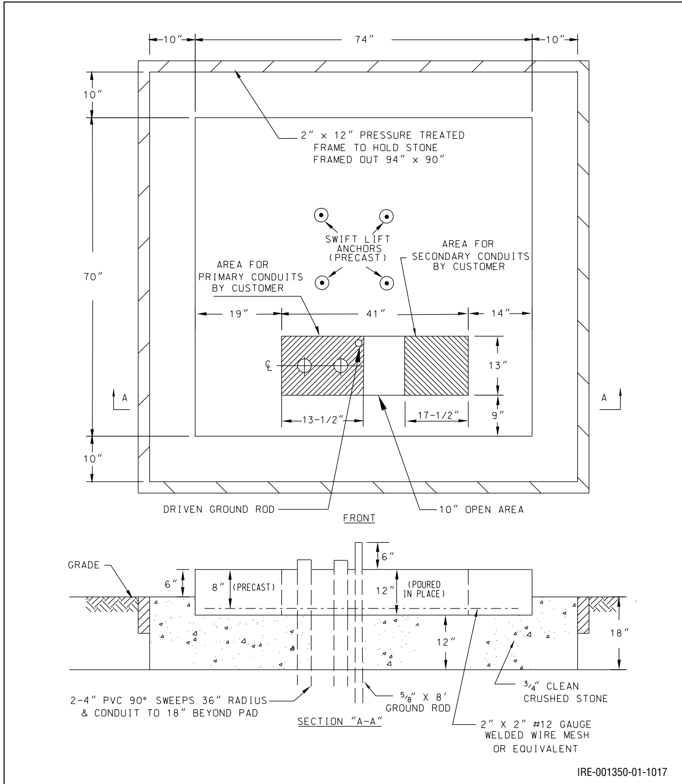
Figure 10.40: Three-Phase Padmounted Transformer – Type II-A (Concrete)
