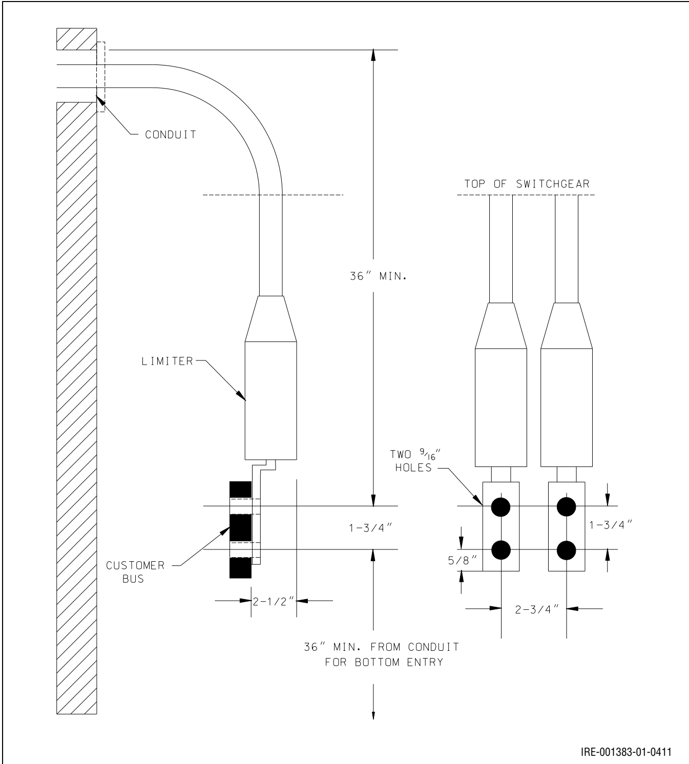
Figure 10.51: Limiter Lug Assembly – 350 MCM and 500 MCM 600 V Rubber Insulated Service Cable
