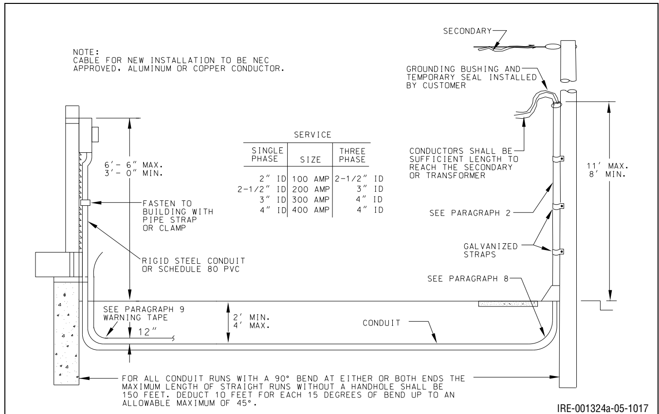
Figure 10.10: Service in Conduit
