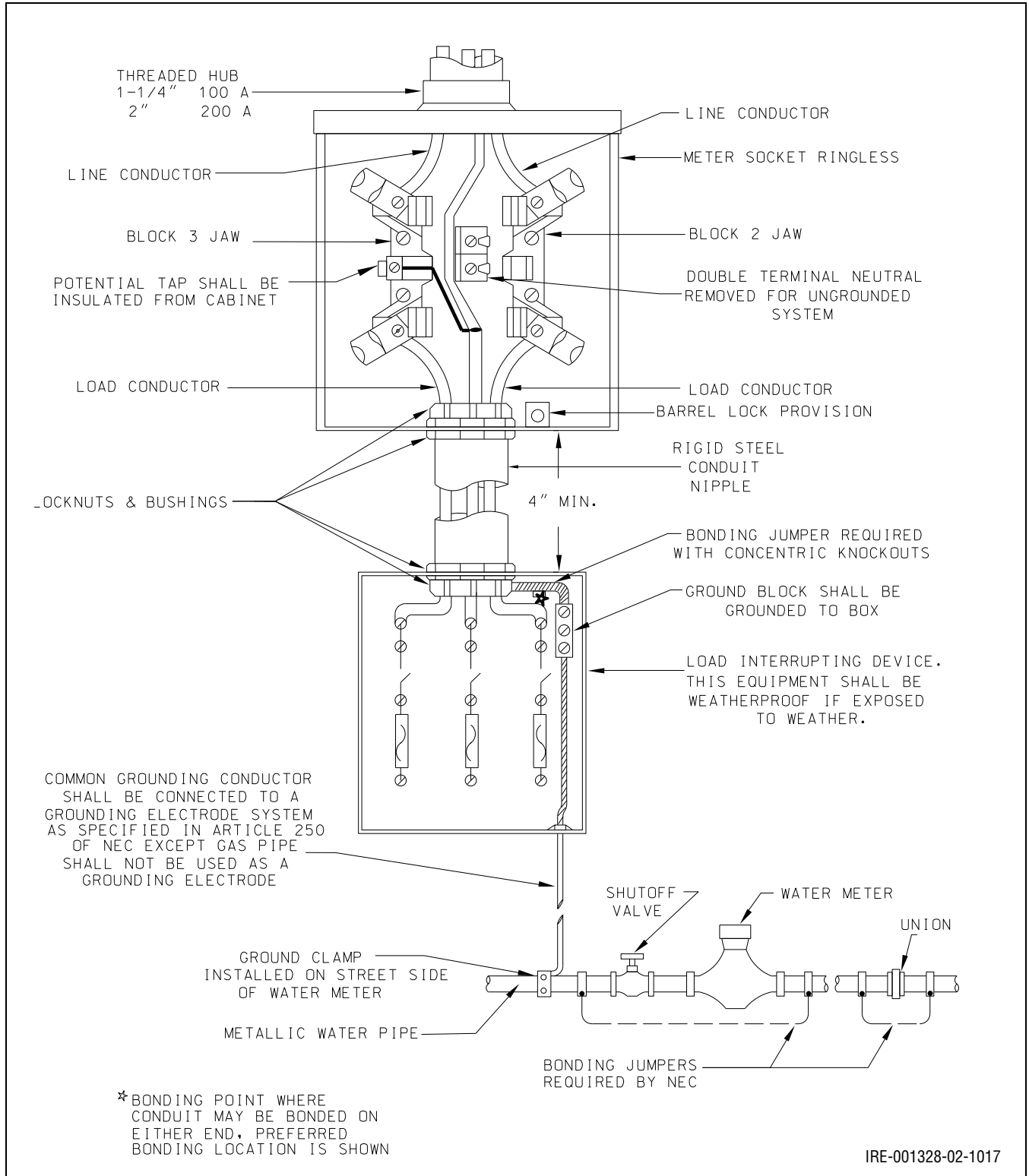
Figure 10.17: Three-Phase, Three-Wire, 240 V Service – Ungrounded System
