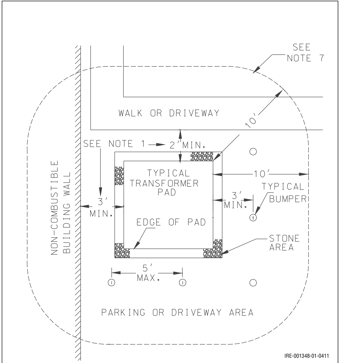
Figure 10.38: Three-Phase Padmounted Transformers
