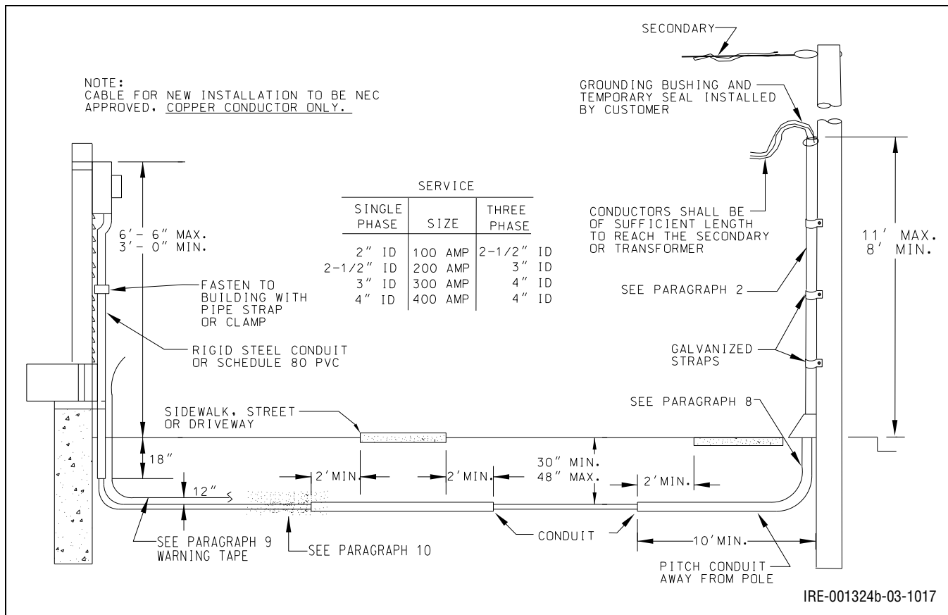
Figure 10.11: Direct Buried Service
