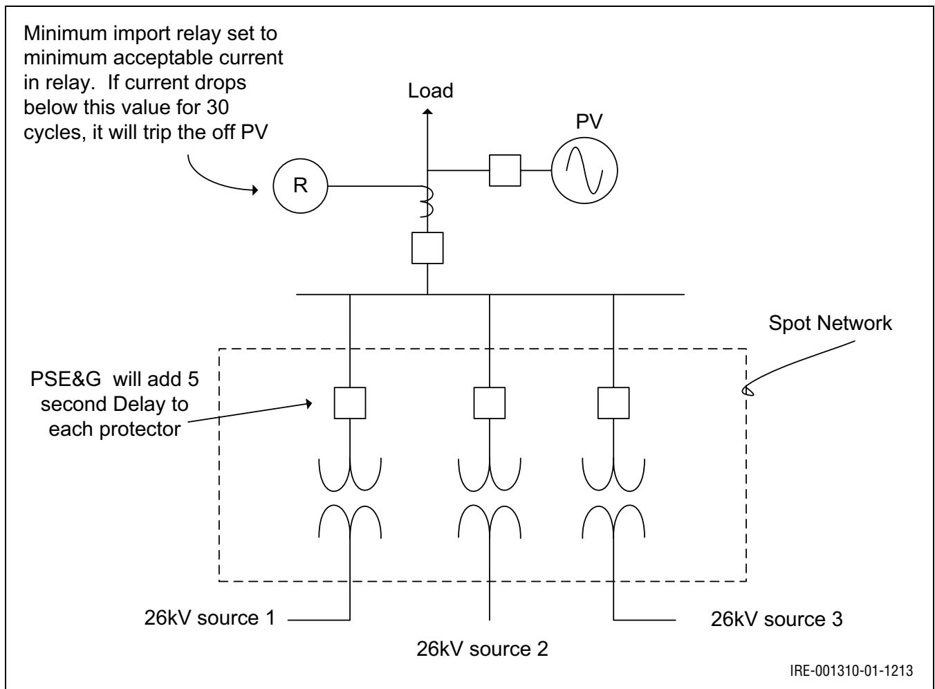
Figure 9.4: Minimum Import Relay
