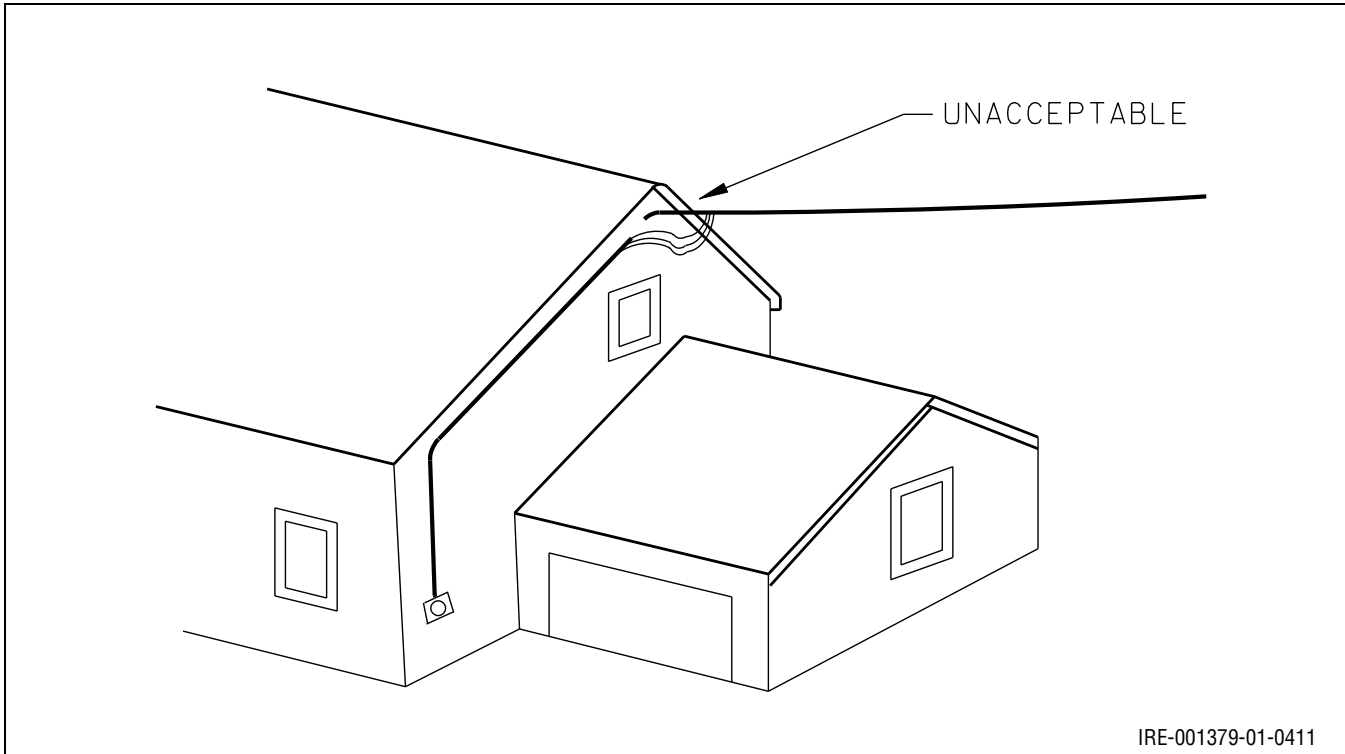
Figure 10.6: Diagram of Typical Installation – Unacceptable Service Location
