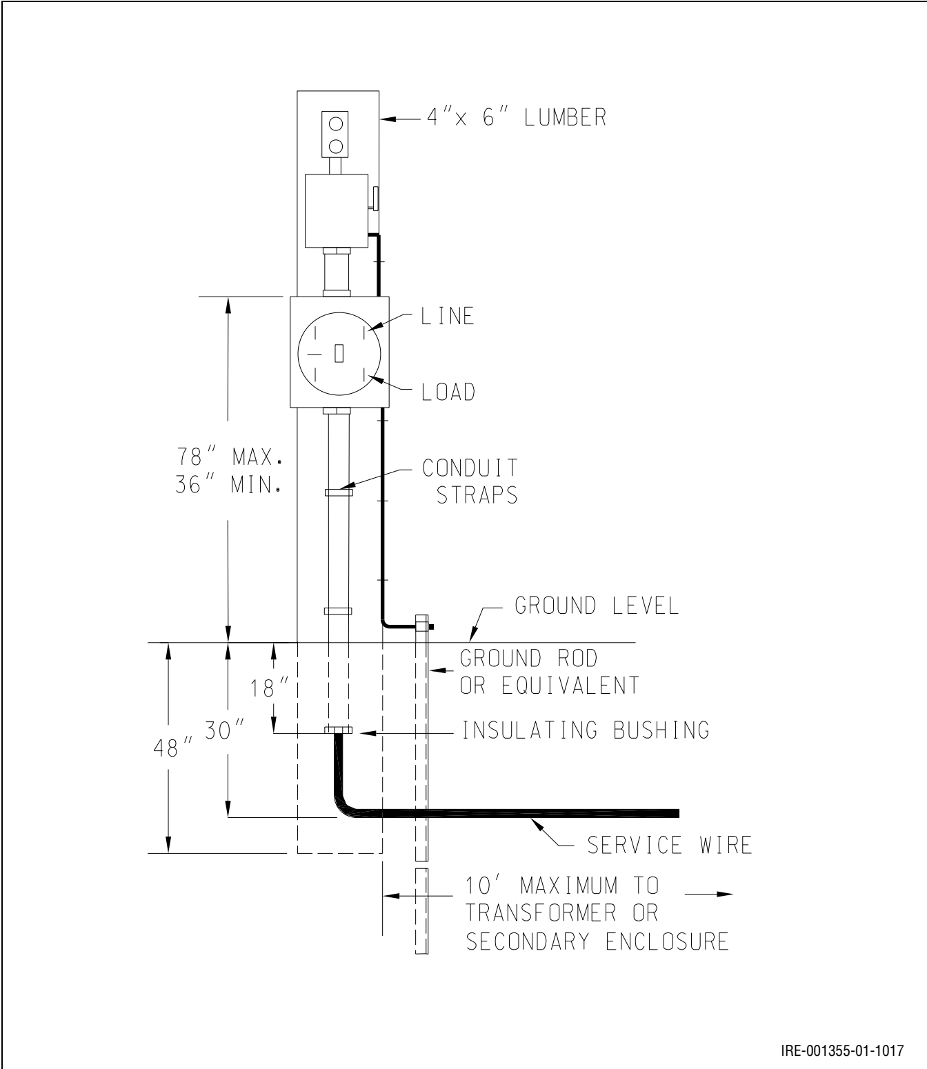
Figure 10.48: Underground Temporary Service Mast
