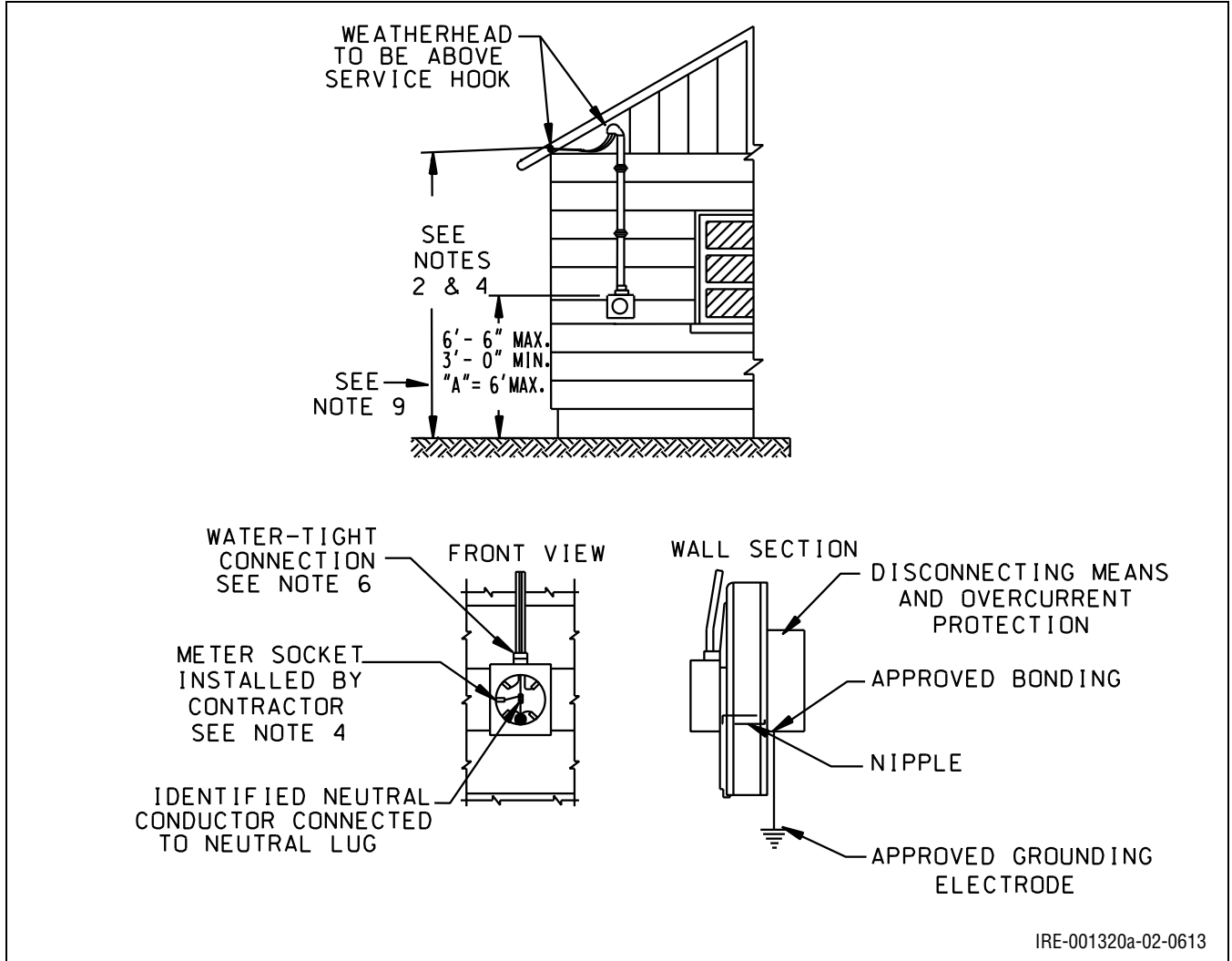
Figure 10.3: First Floor Installation
