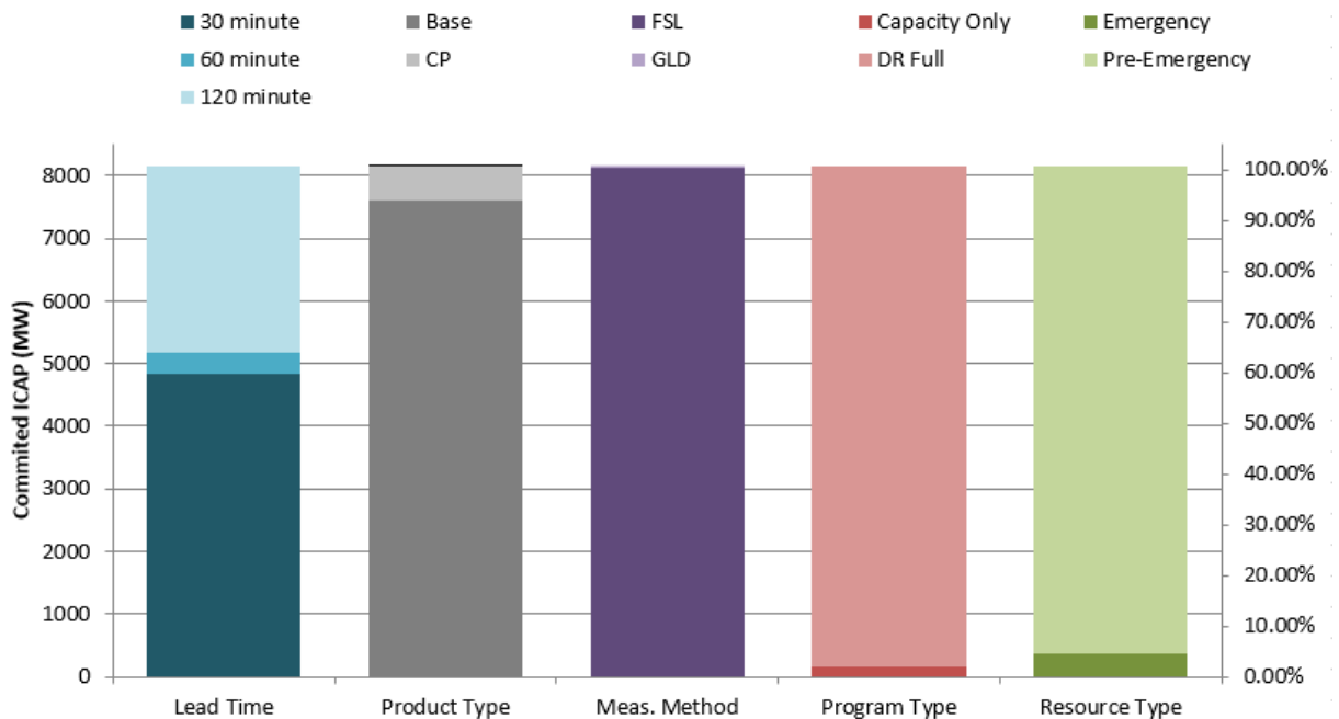
Figure 2: Committed ICAP for DR by Resource Type, Lead Time, Program Type, and Measurement Method for the 2019/20 Delivery Year.
