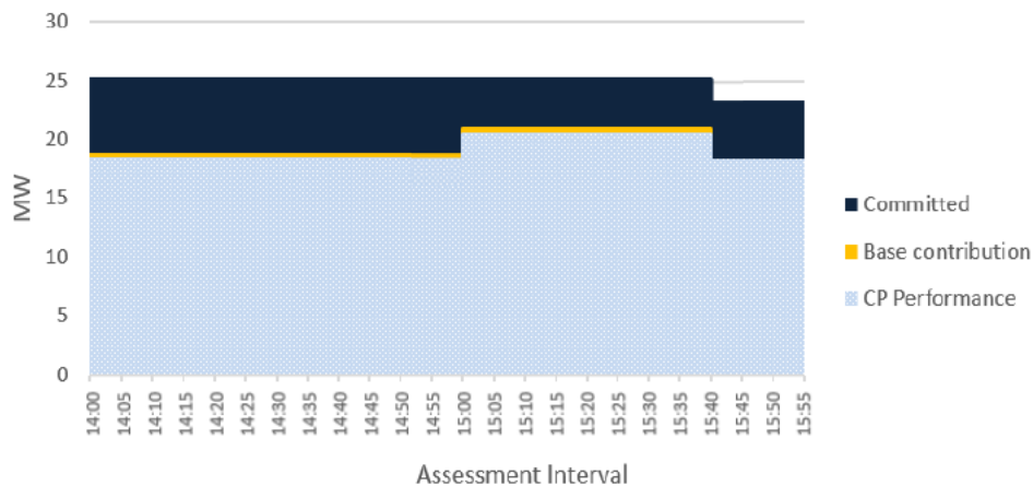
Figure 3. Load Management interval performance during the event
