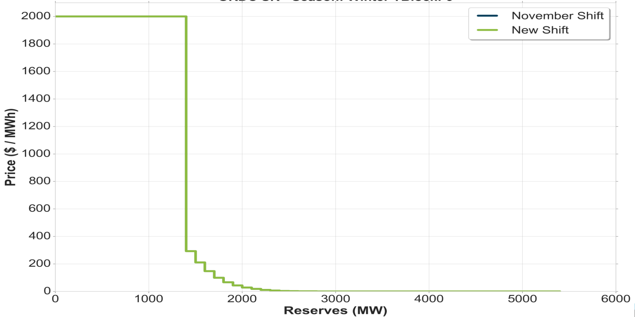
ORDC SR - Season: Winter TBlock: 6
