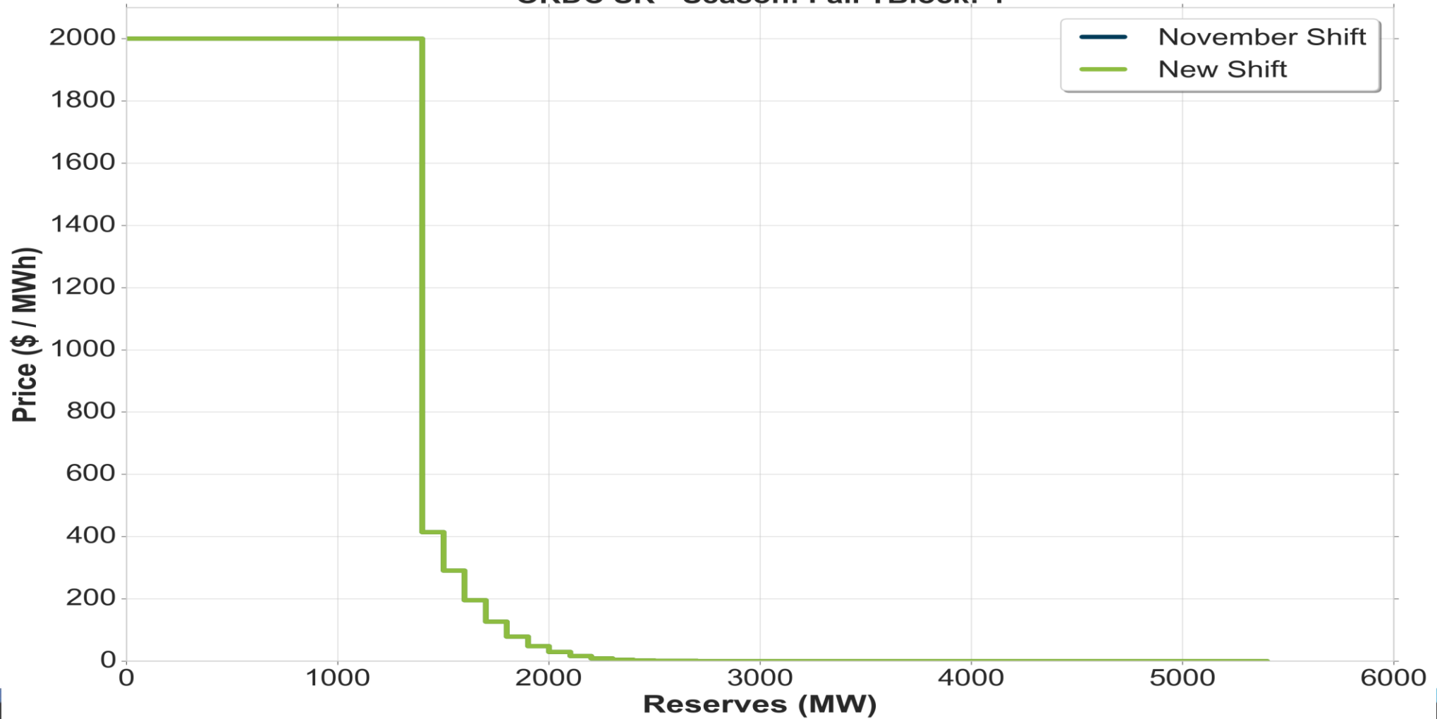
ORDC SR - Season: Fall TBlock: 4
