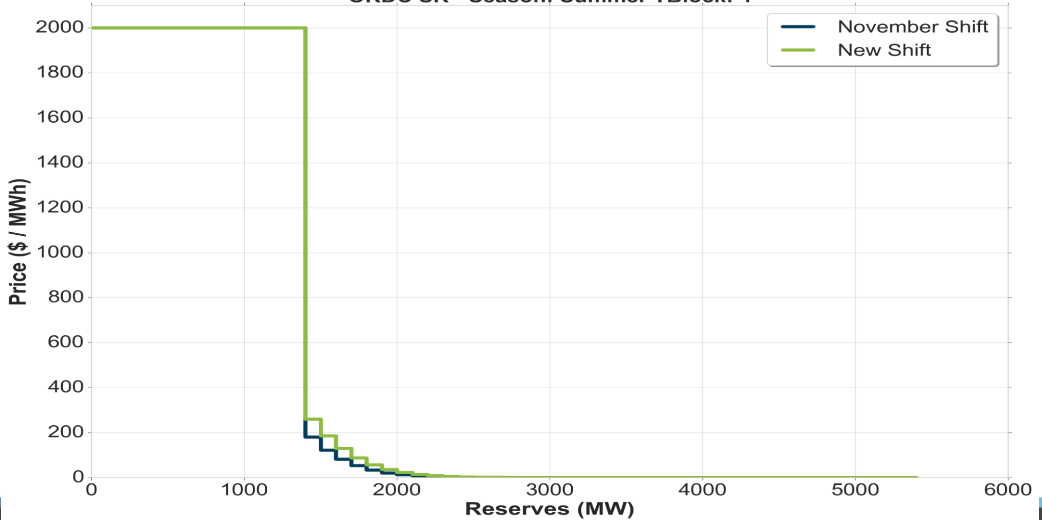
ORDC SR - Season: Summer TBlock: 4
