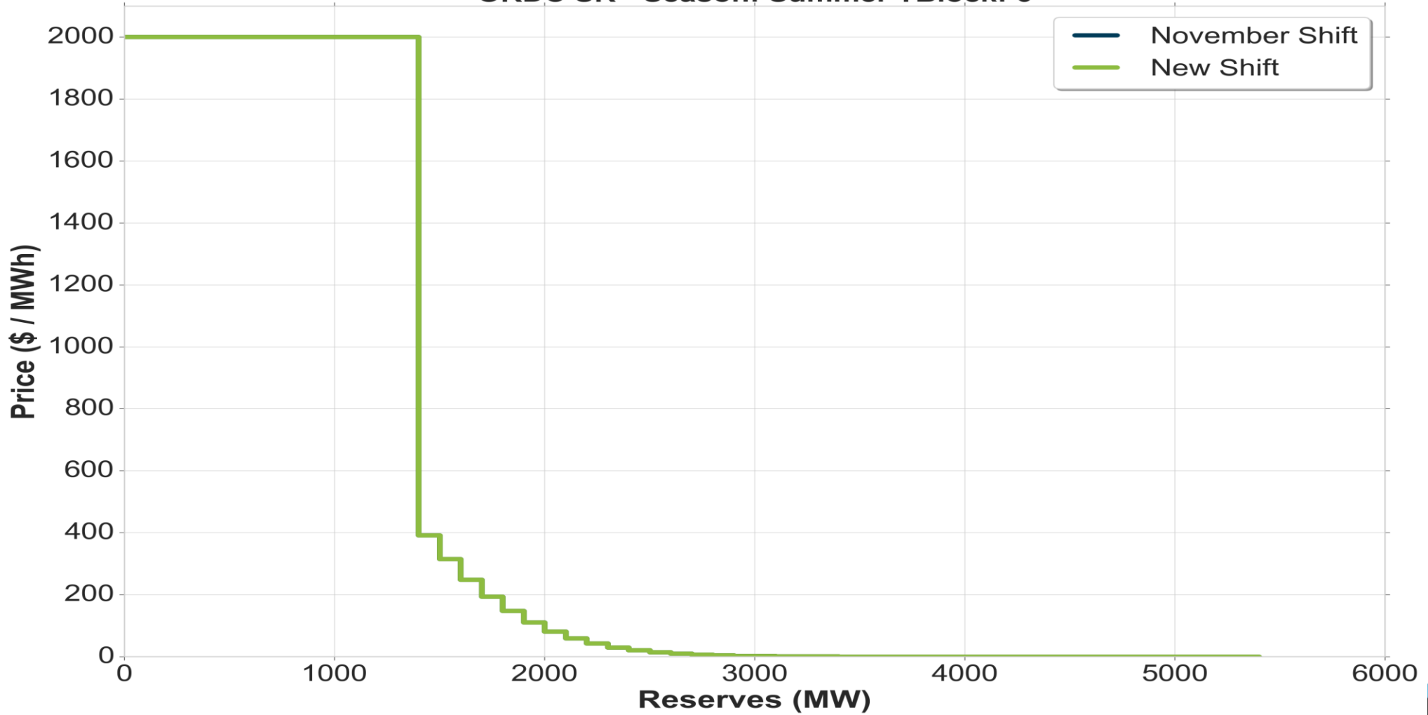
ORDC SR - Season: Summer TBlock: 6
