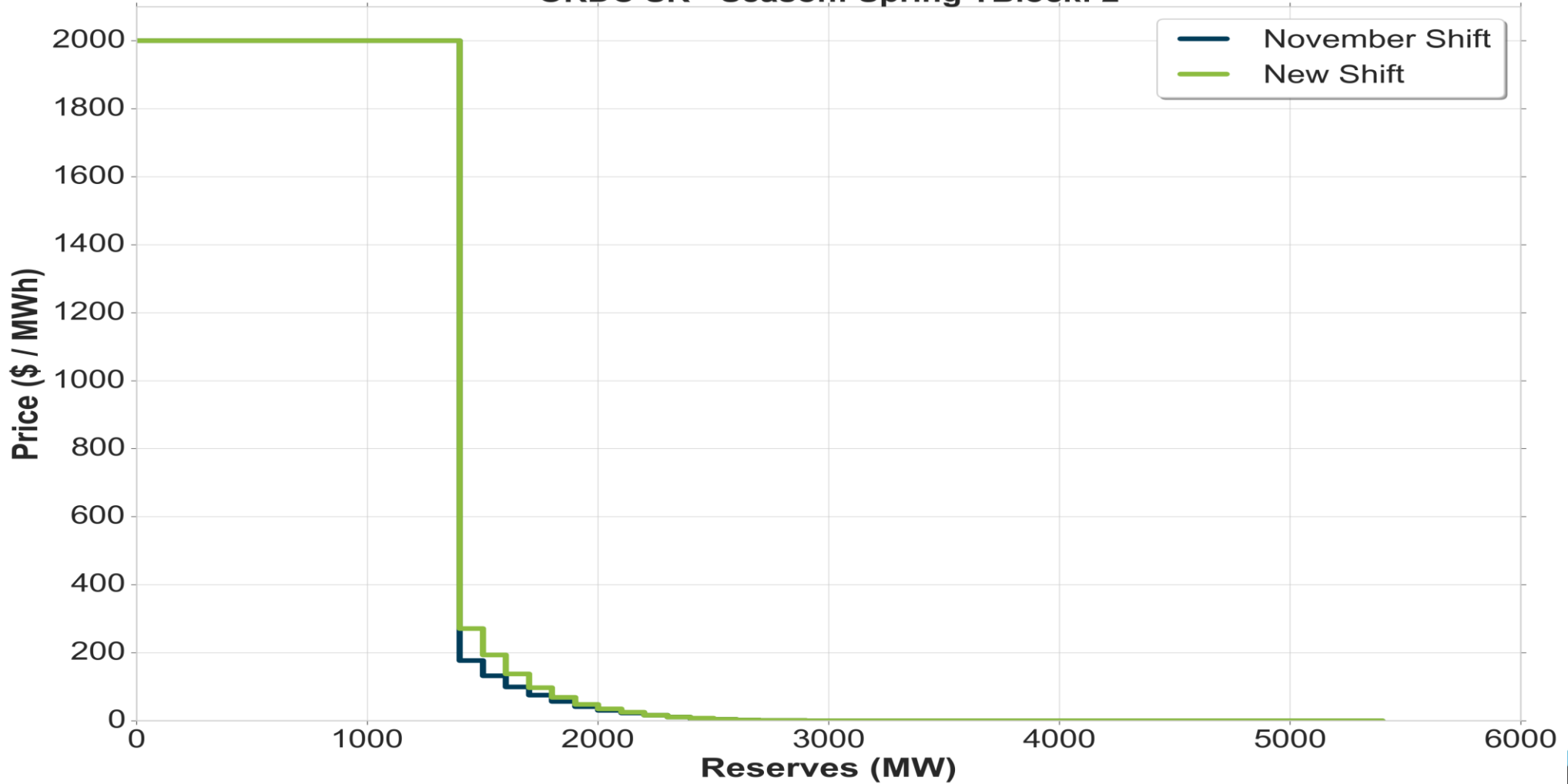
ORDC SR - Season: Spring TBlock: 2
