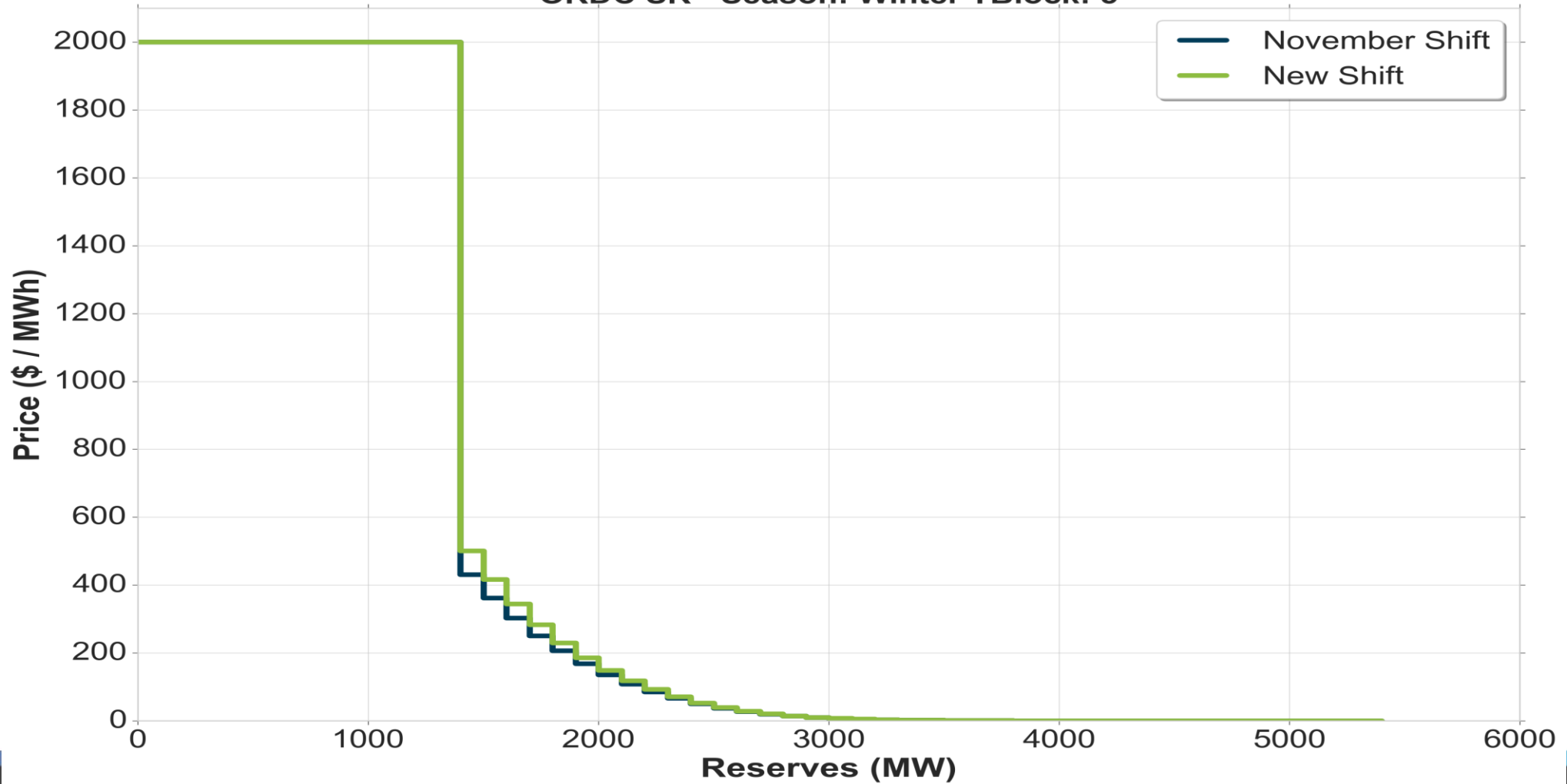
ORDC SR - Season: Winter TBlock: 5
