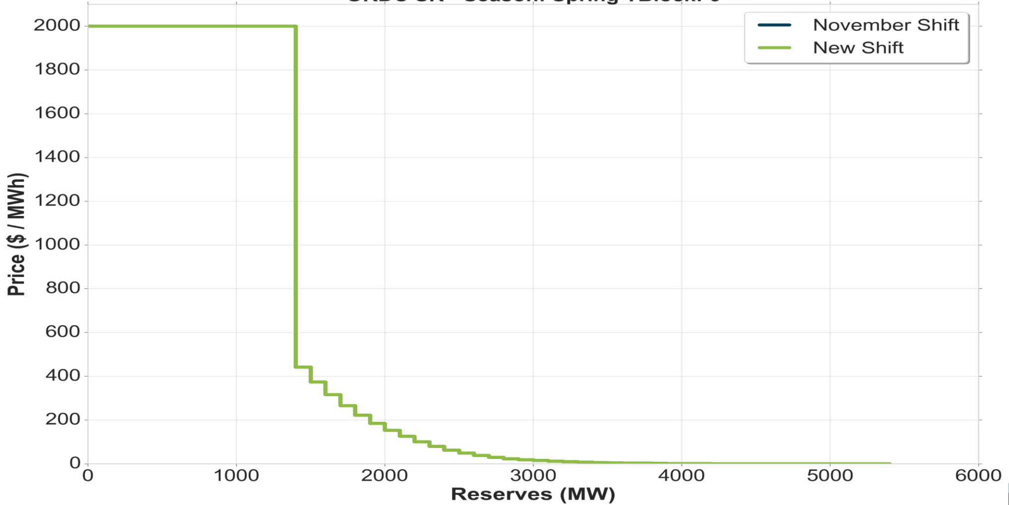
ORDC SR - Season: Spring TBlock: 6
