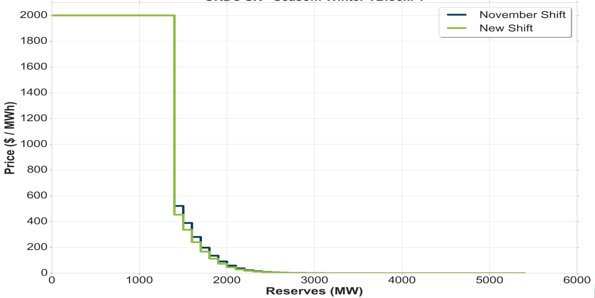
ORDC SR - Season: Winter TBlock: 1
