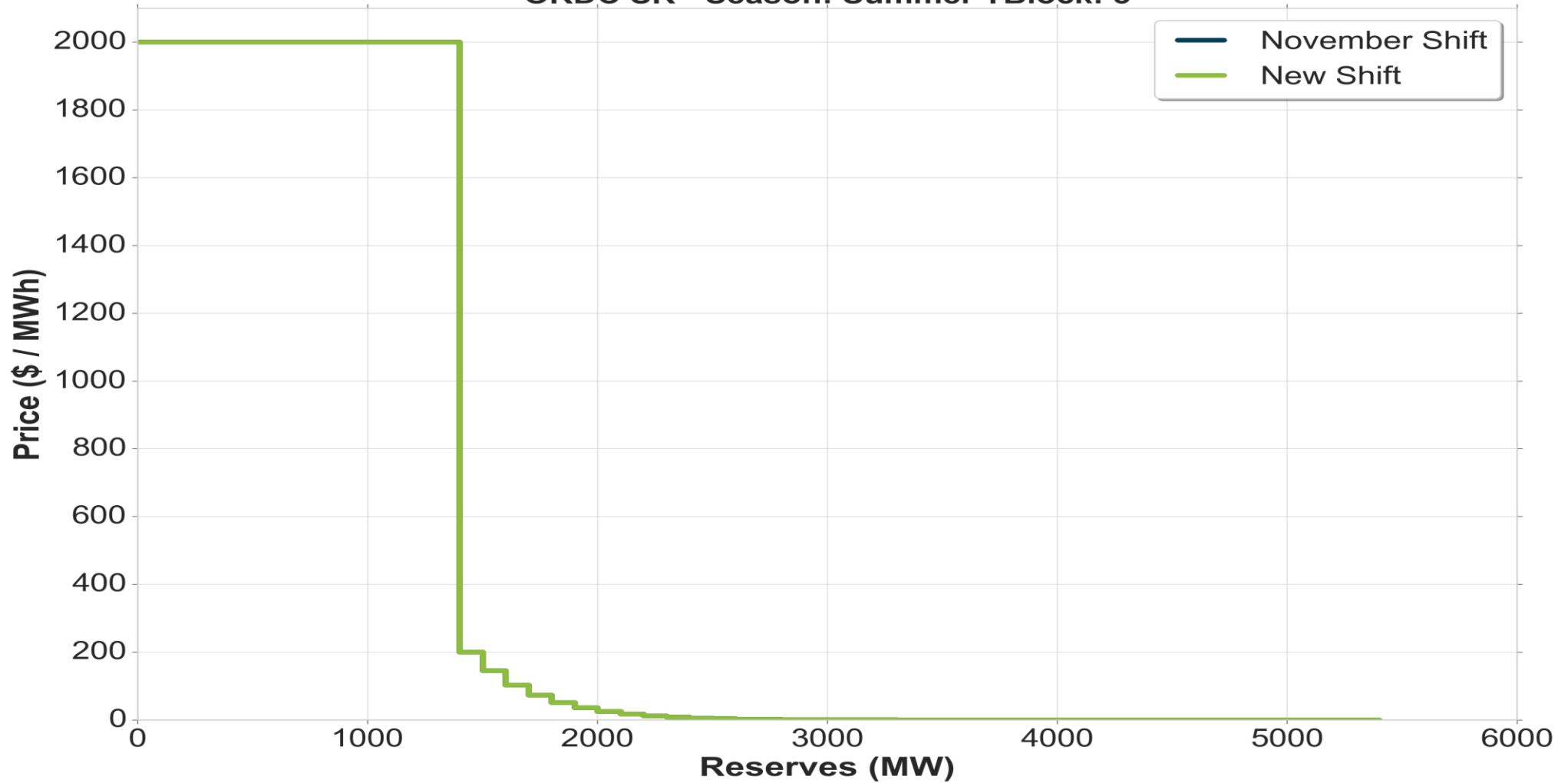
ORDC SR - Season: Summer TBlock: 3
