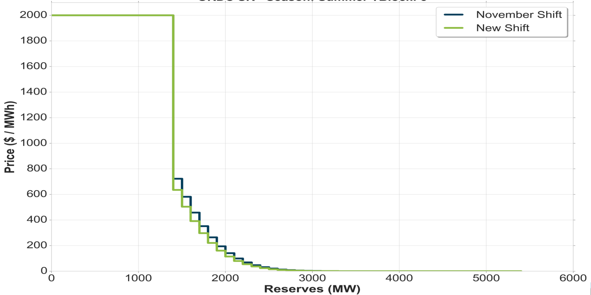
ORDC SR - Season: Summer TBlock: 5
