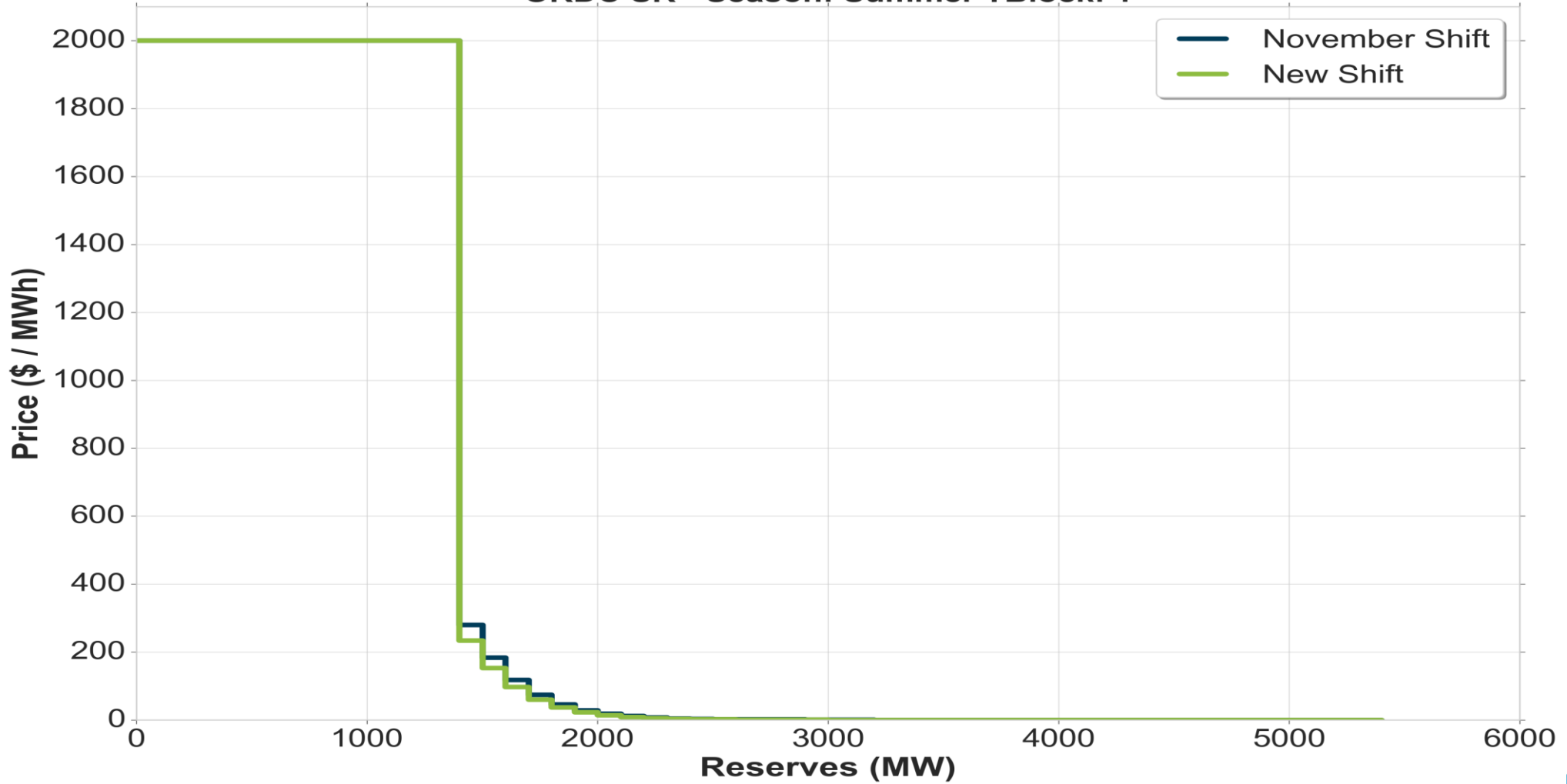
ORDC SR - Season: Summer TBlock: 1
