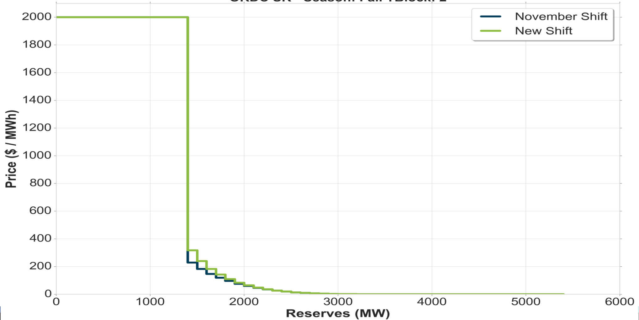
ORDC SR - Season: Fall TBlock: 2
