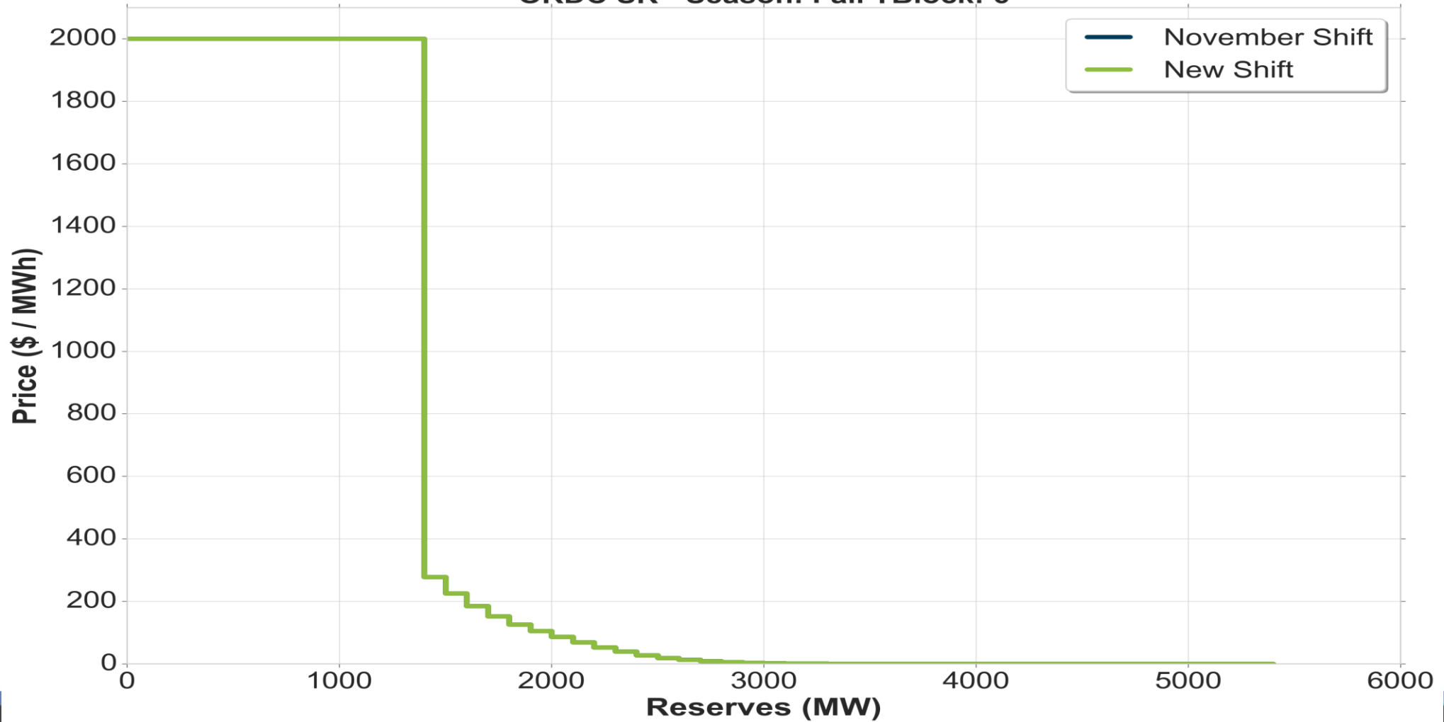
ORDC SR - Season: Fall TBlock: 6
