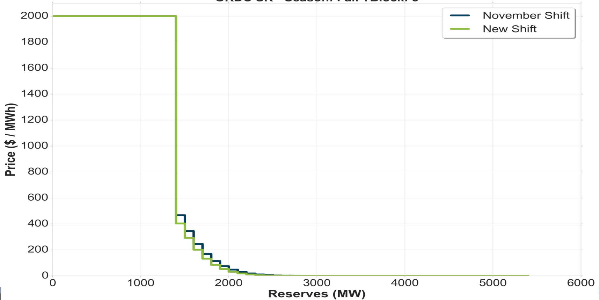
ORDC SR - Season: Fall TBlock: 3
