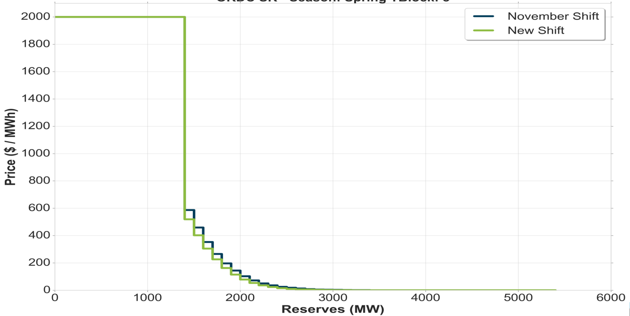
ORDC SR - Season: Spring TBlock: 3
