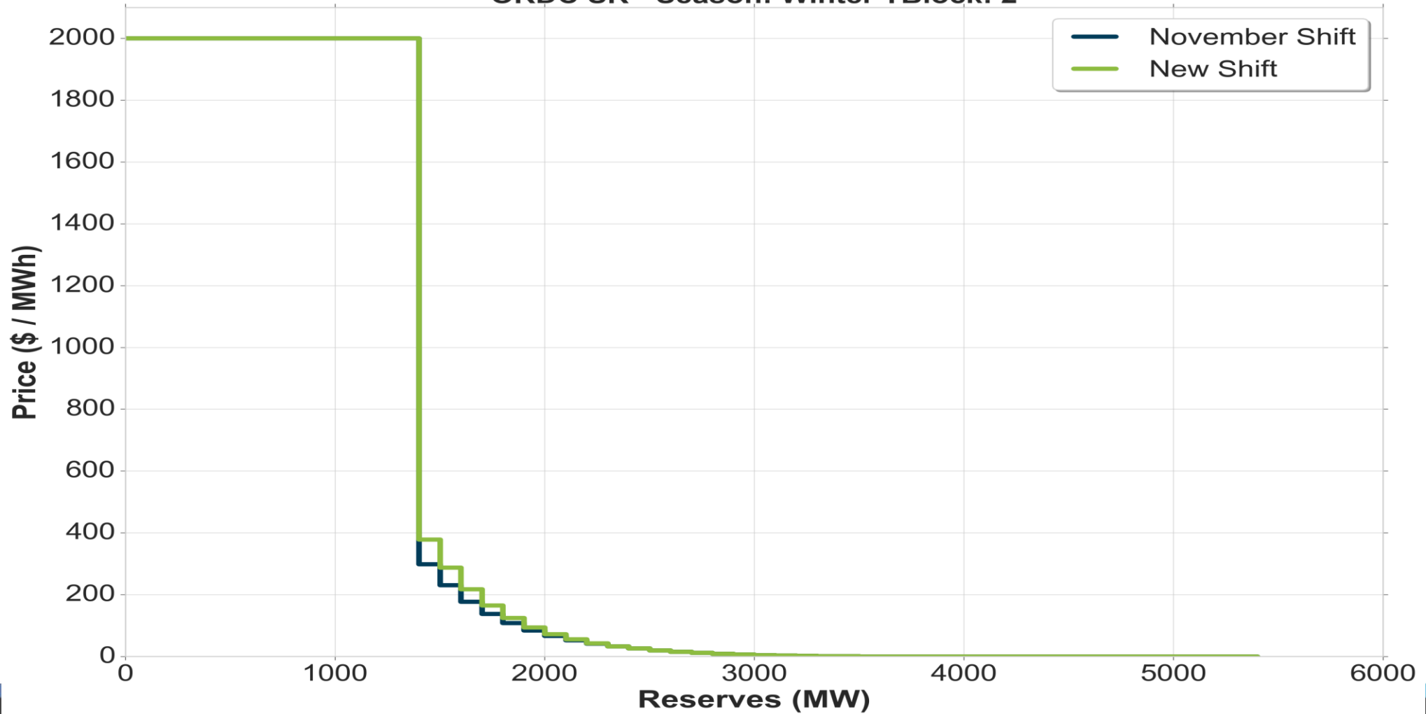
ORDC SR - Season: Winter TBlock: 2
