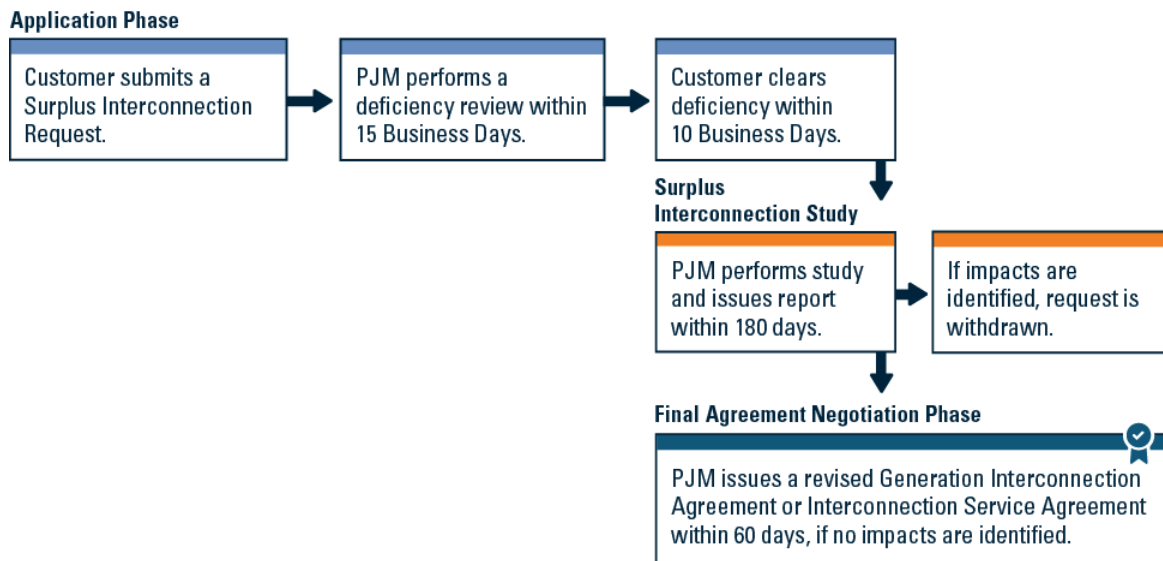
Exhibit 33: Surplus Interconnection Request Process
