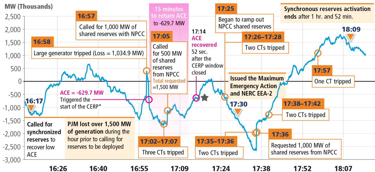
Figure 17. ACE During DCS
