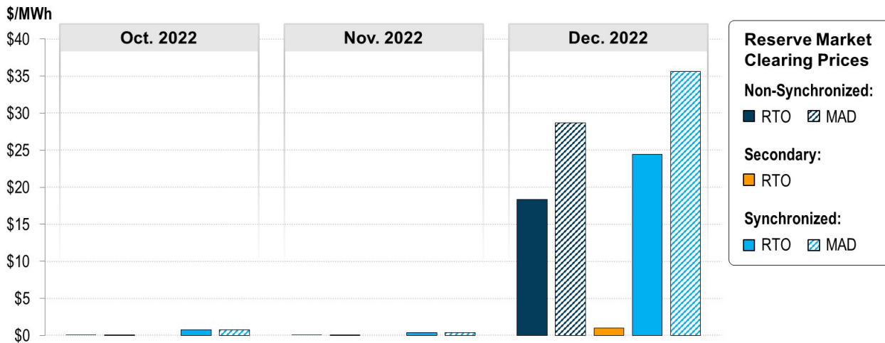
Figure 80. SRMCPs, NSMCPs and SecRMCPs
